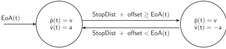
Fig. 8. An abstract train speed controller hybrid automata model with two modes.
