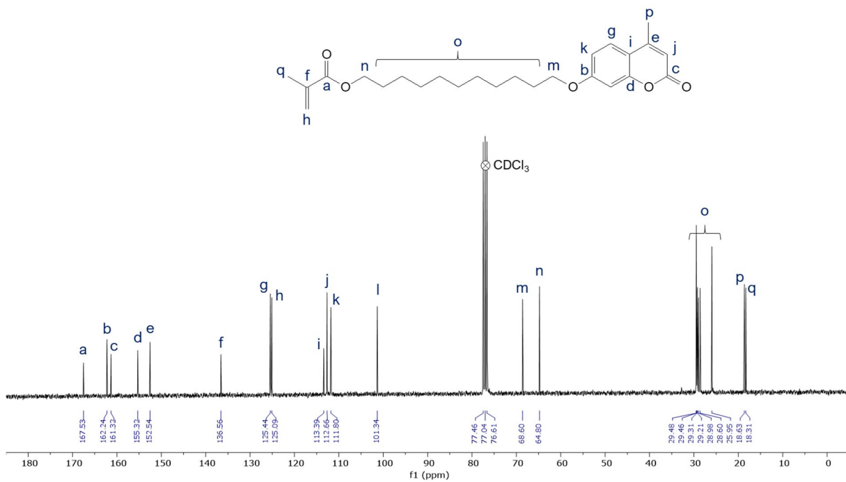
Figure S2. a) 1 H and b) 13 C NMR spectra of CoumMA in CDCl 3 .
