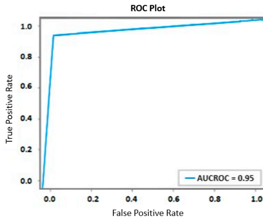
Figure 5. ROC Curve.
