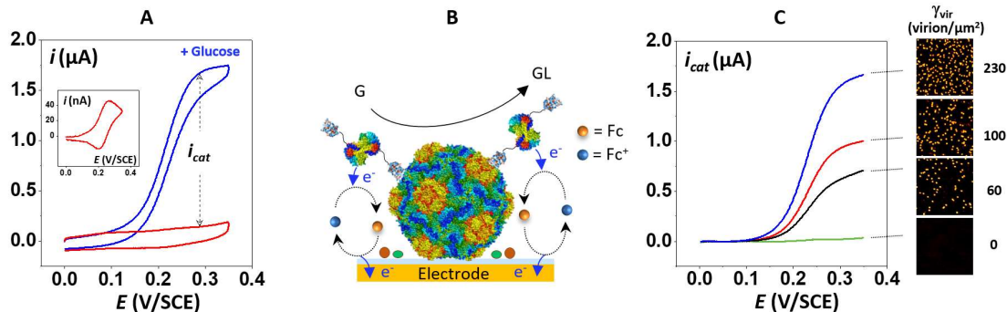
Figure 2. (A) Cyclic voltammograms (CVs) recorded at a TS gold electrode bearing GFLV decorated by the GDH-Nb 75 fusion, in the presence of 3 \mu\text{M} ferrocenedimethanol (Fc), both before (red trace) and after (blue trace) injection of glucose (G) up to a concentration of 3 mM. The inset shows the CV recorded before glucose correction, corrected from the capacitive background current. (B) Schematics of the decorated particles and of the catalytic cycle triggered by glucose injection: the enzyme converts glucose into gluconolactone (GL) using the electrode-produced oxidized form of ferrocenedimethanol ( \text{Fc}^+ ) as a redox co-substrate. (C): CVs recorded in the presence of 3 \mu\text{M} Fc and 3 mM glucose at a TS gold electrode bearing GDH-Nb 75 -decorated GFLV at various surface coverage, \gamma_{\text{vir}} , as indicated. Virus coverages were determined by counting virions from AFM-images, as shown. 50 mM pH = 7.5 Tris-HCl buffer. Potential scan rate = 20 mV/s. T = 25 °C.
