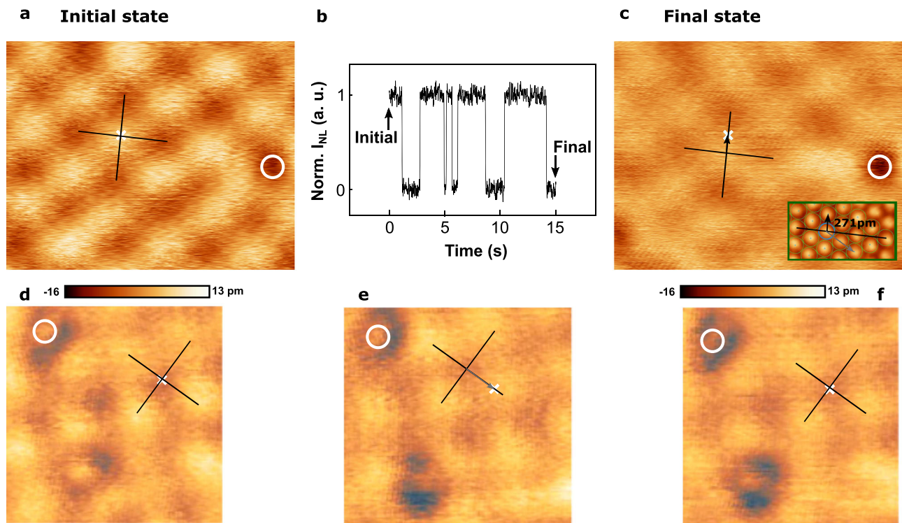
Fig. 5 | STM observation of the sliding phason. a STM image of the initial state where the white circle marks a defect that serves as a reference for the scan area ( U = 10 mV, I = 10 nA). The time trace of panel (b) was recorded with the STM tip positioned at the location of the small white cross. The two black lines indicate the orientations \mathbf{a}_\pm of the crystallographic unit cell, see Fig. 1. b Time trace of the rectified current I_{NL} recorded at the position indicated by the white cross in (a) and (c) with U = 80 mV, I = 20 nA, and an additional ac voltage with amplitude U_{ac} = 27.2 mV at 2 GHz. c STM image of the final state ( U = 10 mV, I = 10 nA). Compared to the initial
