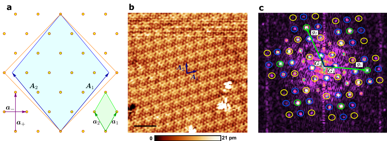
Fig. 1 | Atomic and magnetic structure of Fe/Ir(111). a Atomic and magnetic Bravais lattices of Fe/Ir(111). Yellow dots represent the hexagonal lattice of Fe atoms, with a unit cell given by the green-shaded rhombus and primitive vectors \mathbf{a}_1 and \mathbf{a}_2 , with \mathbf{a}_\pm = \mathbf{a}_1 \pm \mathbf{a}_2 . The blue-shaded rhombus is a primitive unit cell of the magnetic order, with primitive vectors \mathbf{A}_1 and \mathbf{A}_2 . The magnetic order possesses a uniaxial commensurability, \mathbf{A}_1 + \mathbf{A}_2 = 3\mathbf{a}_+ . The orange lines represent the 3 × 5 commensurate approximation of the magnetic unit cell. b Atomically resolved spin-polarized STM image of the magnetic order ( U = 10 \text{ mV} , I = 15 \text{ nA} ) on Fe/Ir(111). The primitive vectors of the magnetic order of panel (a) are also indicated. The
