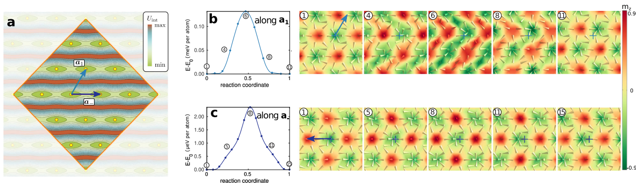
Fig. 3 | Geodesic nudged elastic band calculations. a Illustrative sketch of the effective potential for the sliding phason mode for the 3 × 5 commensurate magnetic texture of Fig. 2, see “Methods” for details. b, c Geodesic nudged elastic band calculations for a shift of the magnetic texture along the \mathbf{a}_+ and \mathbf{a}_- directions, respectively. The panels on the left- and right-hand side depict, respectively, the energy per
