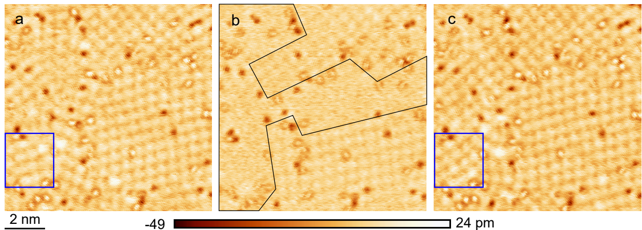
FIG. 4. a. Topographic STM image of the magnetic texture observed at bias voltage U=10 mV and tunneling current I=10 nA. b. The same area scanned at an elevated bias voltage of U=100 mV where the magnetic texture appears to be blurred within the region marked by black lines. c. The subsequent image recorded at U=10 mV shows again a static texture where minor modifications with respect to panel a can be spotted, e.g., in the area marked by the blue box. The legend indicates the colour code of the topographic height.
