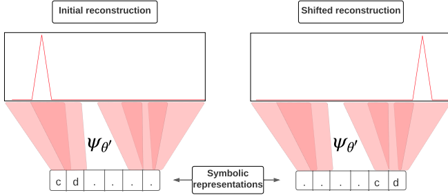
Fig. 4. Shift equivariance of \psi_{\theta'} . The subsequence c d appear at two different locations in the representation: \psi_{\theta'} should decode the same pattern with a shift in time.
