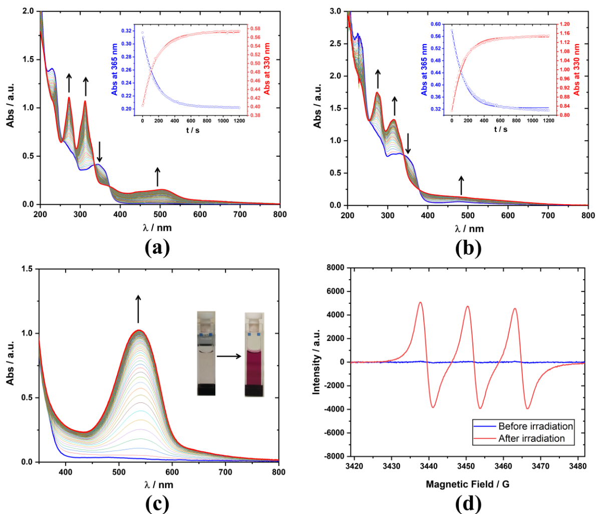
Figure 5. Spectral evolution at 25 °C under irradiation at \lambda = 365 nm during 20 min for (a) acac-RuNO (6a) , 3.54 \times 10^{-5} M in acetonitrile, I_0 = 6.22 \times 10^{-6} \text{ molL}^{-1}\text{s}^{-1} ) and (b) 7a ( 7.31 \times 10^{-5} M in water, I_0 = 6.35 \times 10^{-5} \text{ molL}^{-1}\text{s}^{-1} ); inset shows fitting of the photokinetic data at two wavelengths, with average correlation coefficients R^2 = 0.995 and 0.993 , respectively. Below are representative experiments on 7a that demonstrate NO release in water under irradiation at \lambda = 365 nm, as evidenced from (c) the formation of an azo dye in the presence of the Griess reagent 61 and (d) the observation of an EPR signal using the NO-selective [\text{Fe}^{\text{II}}(\text{MGD})_2] spin trap; with a g -factor of 2.040 and a hyperfine coupling constant, a_{\text{N}} = 1.20 \times 10^{-3} \text{ cm}^{-1} , the observed triplet EPR signal corresponds to a nitric oxide radical. 62
