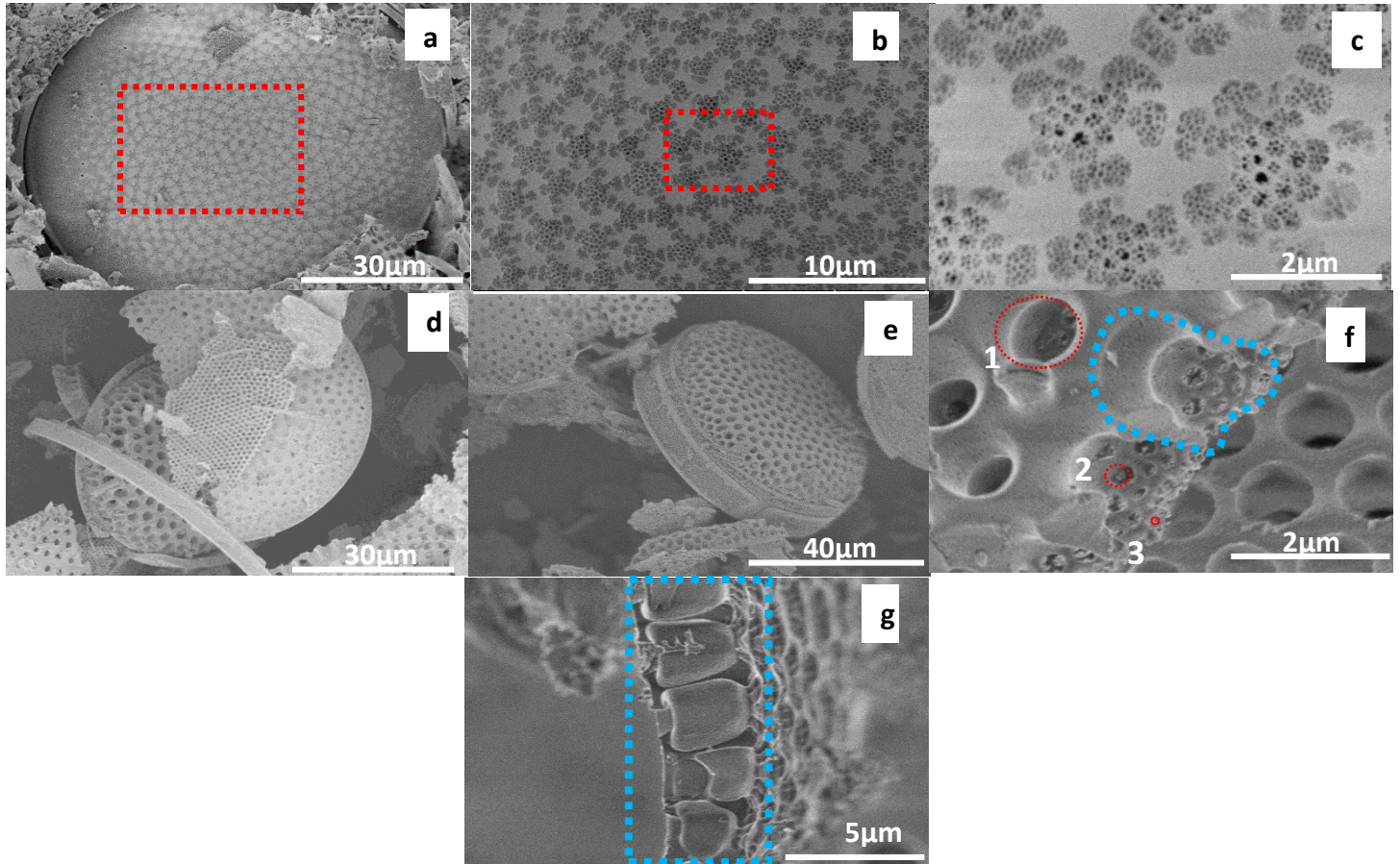
Figure 4: SEM images of diatomite raw rock (a, b, c) and its purified sample S1 after purification protocol (d, e, f, g), (images by Hitachi SU8010)
