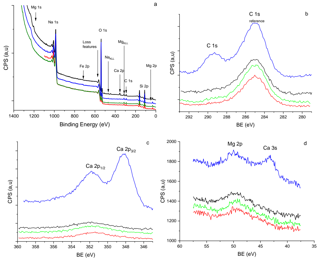
Figure 6: Overview XPS spectra (a) C 1s (b), Ca 2p (c) and Mg 2p (d) core level spectra of diatomite raw rock (blue), S1 (black), S2 (red) and S3 (green)
