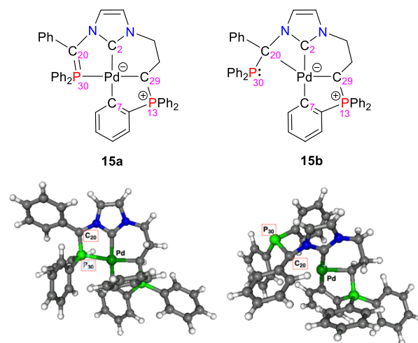
Scheme 7. Calculated Structures of Two Possible Isomers of Pd(II) Complex 15 at PBE-D3/6-31G**/LANL2DZ*(Pd) Level of Calculation (Atoms Color Code: C – grey, N – blue, P – green, Pd – Dark Green.).
