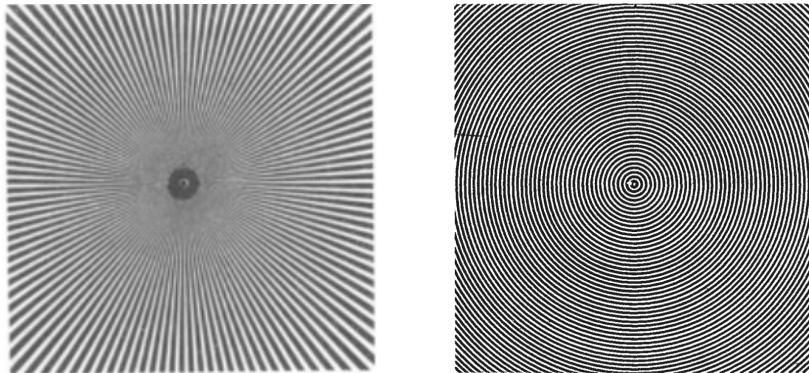
FIGURE 2. The stimuli used in [18]. Left : “MacKay-rays”. Right : “MacKay-target”.
