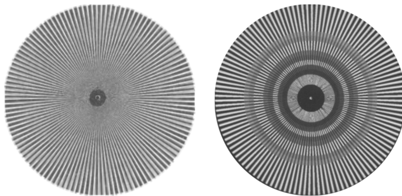
FIGURE 1. The MacKay effect [18], showcasing the illusion induced by the stimulus on the left, referred to as “MacKay rays”. This stimulus leads to an illusory perception of concentric rings superimposed in its background, as illustrated on the right (artist’s depiction by Isia Leviant [17]). To see the illusory contours, look at the centre of the black circle in the image on the left . The adaptation of this figure is based on the original representation from [18, Fig. 1] and [34, Fig. 1b].
