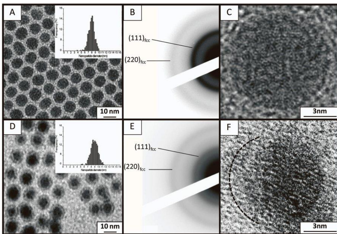
Figure 2. (A) TEM image of 7.9 nm Co fcc nanoparticles, (B) corresponding electron diffraction pattern and (C) HRTEM image of a single nanoparticle. (D) TEM image of 8.8 nm Co fcc @CoO nanoparticles, (E) corresponding electron diffraction pattern and (F) HRTEM image of a single nanoparticle.
