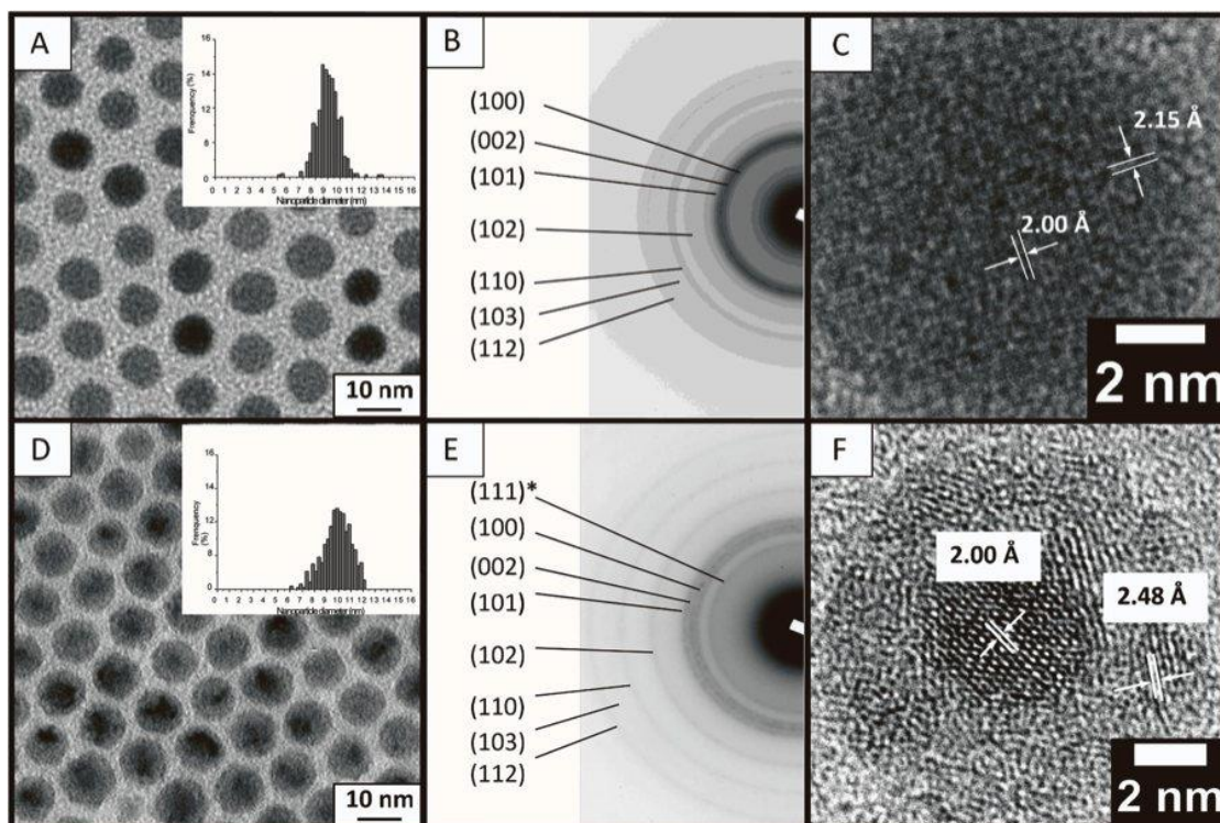
Figure 3. (A) TEM image of 9.0 nm Co hcp nanoparticles, (B) corresponding electron diffraction pattern and (C) HRTEM image of a single nanoparticle. (D) TEM image of 9.9 nm Co hcp @CoO nanoparticles, (E) corresponding electron diffraction pattern and (F) HRTEM image of a single nanoparticle.
