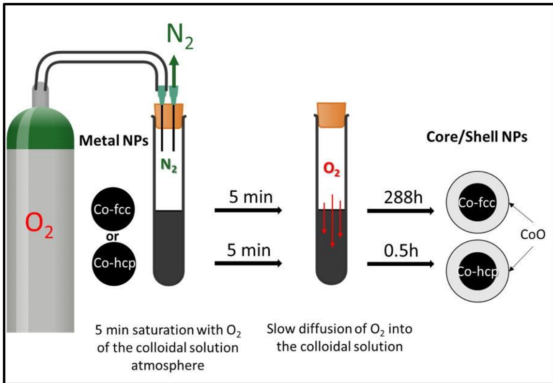
Figure 1. Schematic diagram of the preparation process of \text{Co}@\text{CoO} core/shell nanoparticles.
