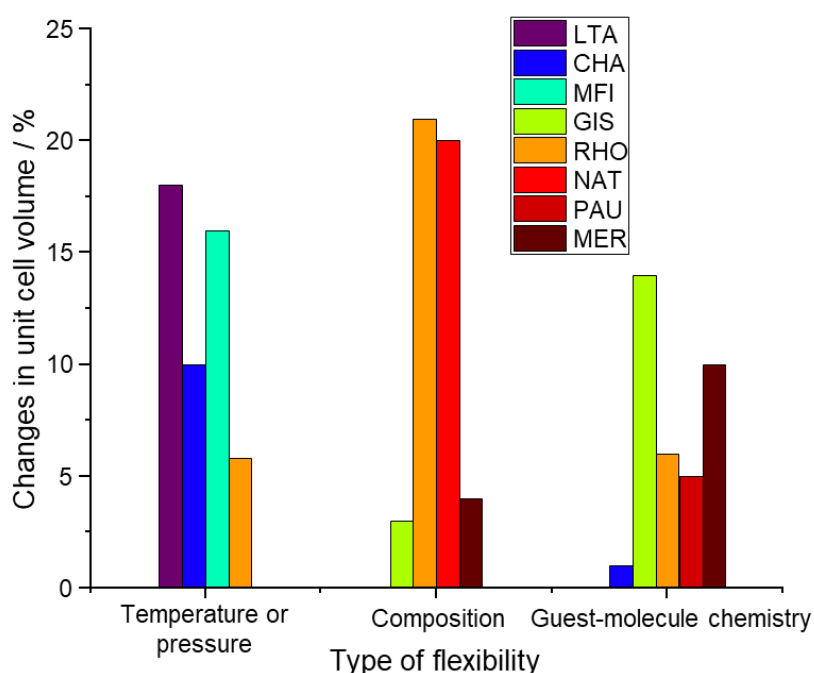
Fig. 8. Maximum changes in the unit cell volume of the most flexible zeolite structures presented in literature. 5,33,37,41-43,46,61,96,98,101,122,125,126
