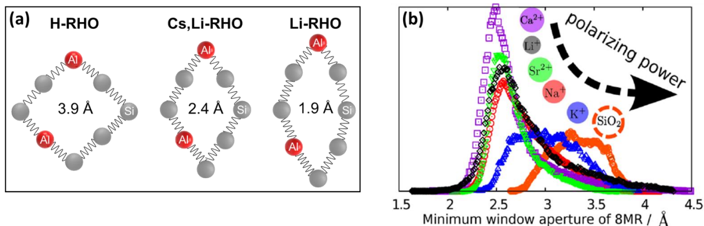
Fig. 7. Ellipticity of zeolite RHO containing different cations (a) based on experiments and (b) based on simulations (adopted with permission from 5 and 123 , copyright 2015 and 2016 American Chemical Society).
