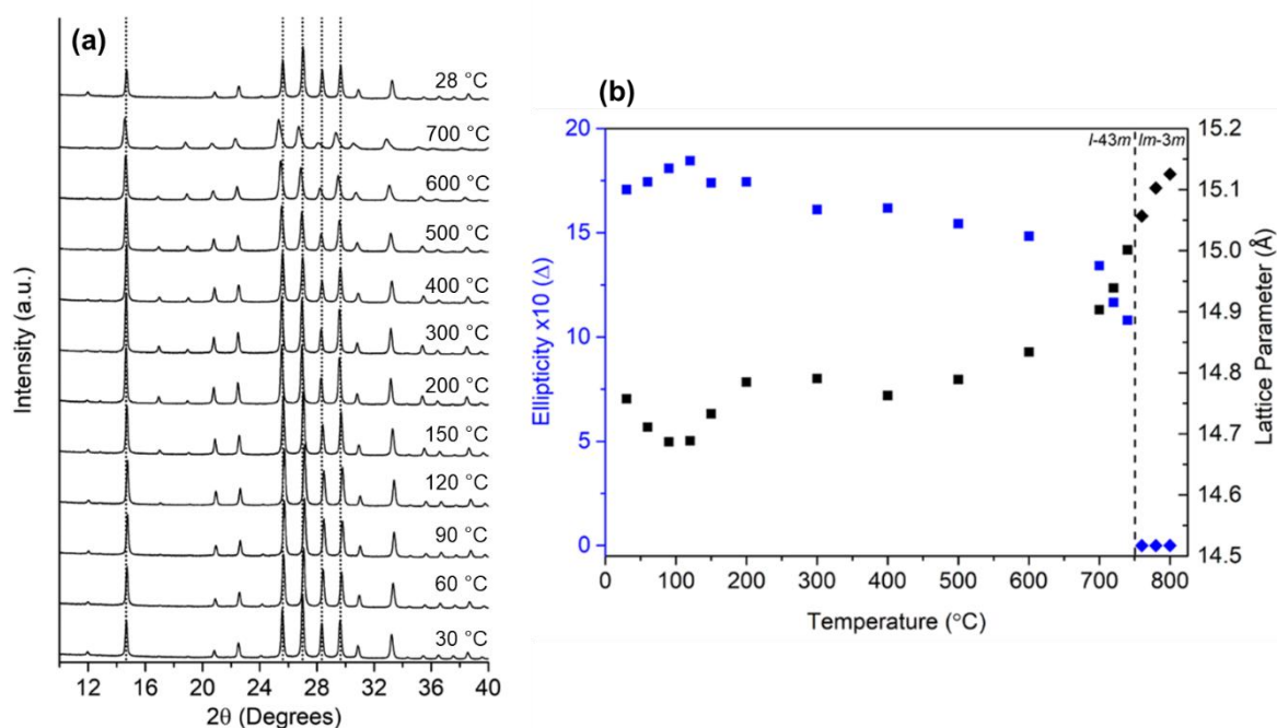
Fig. 1. (a) In-situ variable-temperature XRD scans of nanosized RHO zeolite from 30 to 700 °C and back to 28 °C, (b) plot of the ellipticity of eight-membered ring opening (in blue) and the lattice parameter (black). The dashed line delineates the adoption of either the acentric (squares) or centric (diamonds) space groups (reprinted with permission from 43, copyright 2022 American Chemical Society).
