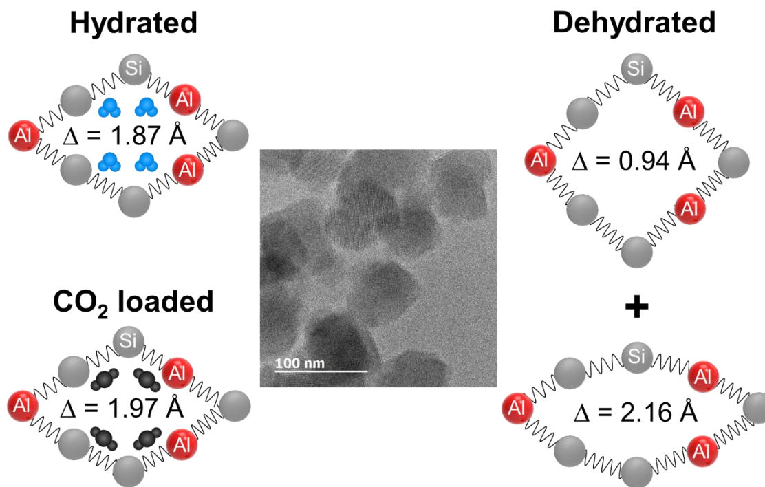
Fig. 5. Schematic illustration of reversible ellipticity of RHO nanosized zeolites upon dehydration and CO 2 adsorption (adopted with permission from 9, copyright 2020 American Chemical Society).
