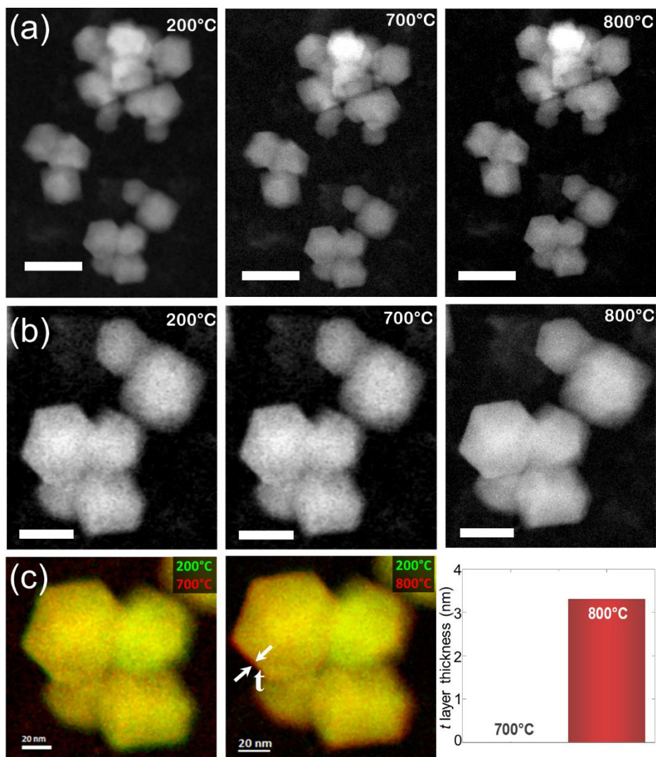
Fig. 2. (a, b) High-angle annular dark-field scanning transmission electron microscopy (HAADF-STEM) analysis of the nanosized RHO submitted to thermal treatment between 200 and 800 °C at different magnifications. Scale bars of 50 and 20 nm for the first and second rows, respectively. (c) Superimposed micrographs acquired at different temperatures show the volume expansion of the region highlighted by red color and denoted by t (adopted with permission from 32, copyright 2023 American Chemical Society).
