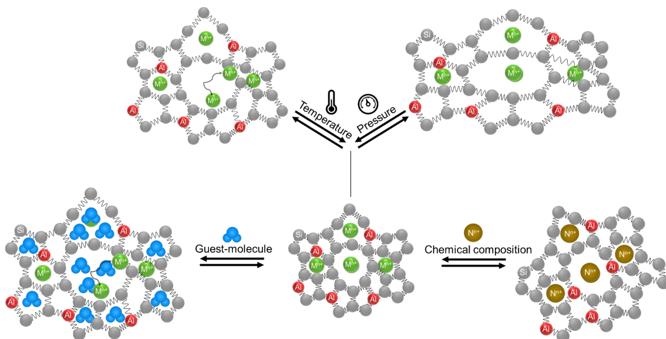
Fig. 3. Schematic illustration of temperature and pressure-induced, guest-induced, and compositionally-induced flexibility in zeolites ( \text{M}^{n+} and \text{N}^{n+} are two arbitrary cations assuming smaller cationic diameter for \text{M}^{n+} compared to \text{N}^{n+} ).
