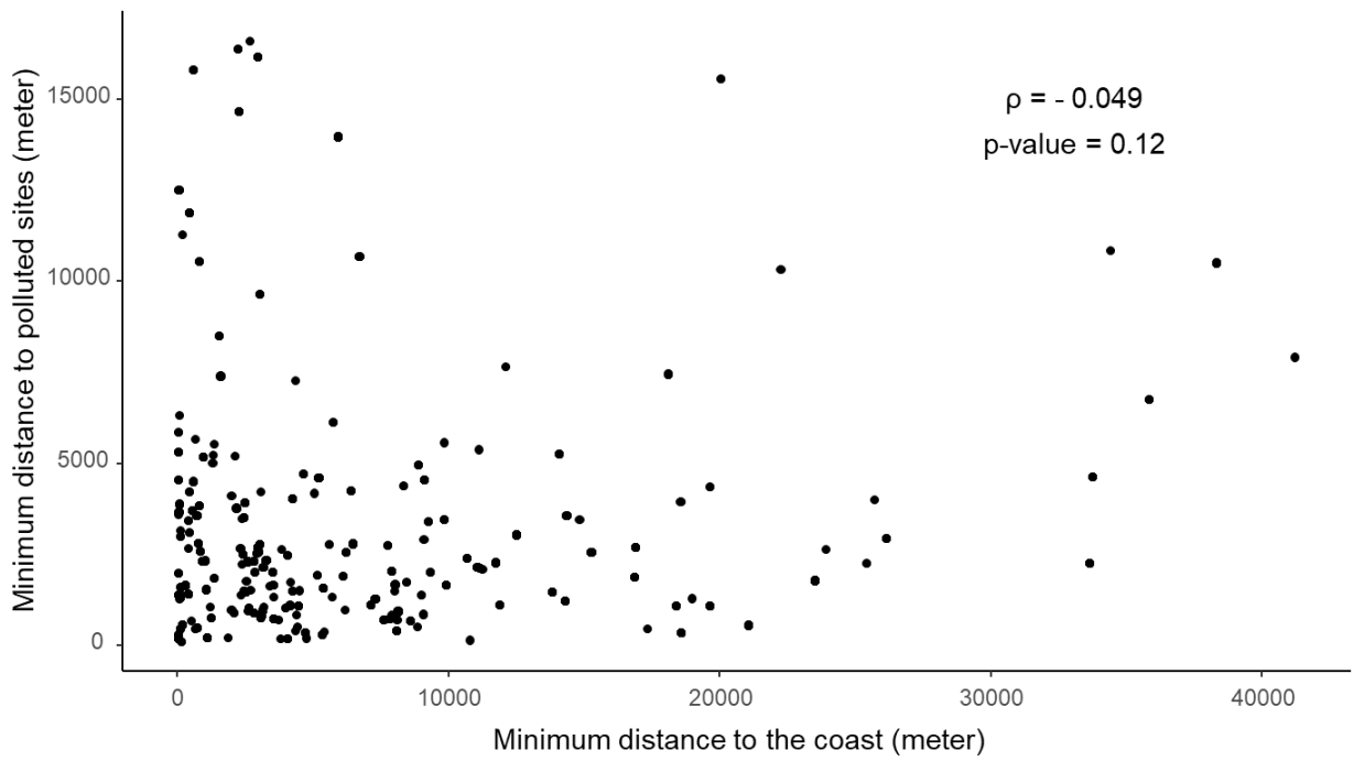
Figure A1. Relation between the minimum distance to polluted sites and the minimum distance to the coast in the full dataset ( \rho : Spearman's coefficient of correlation)
