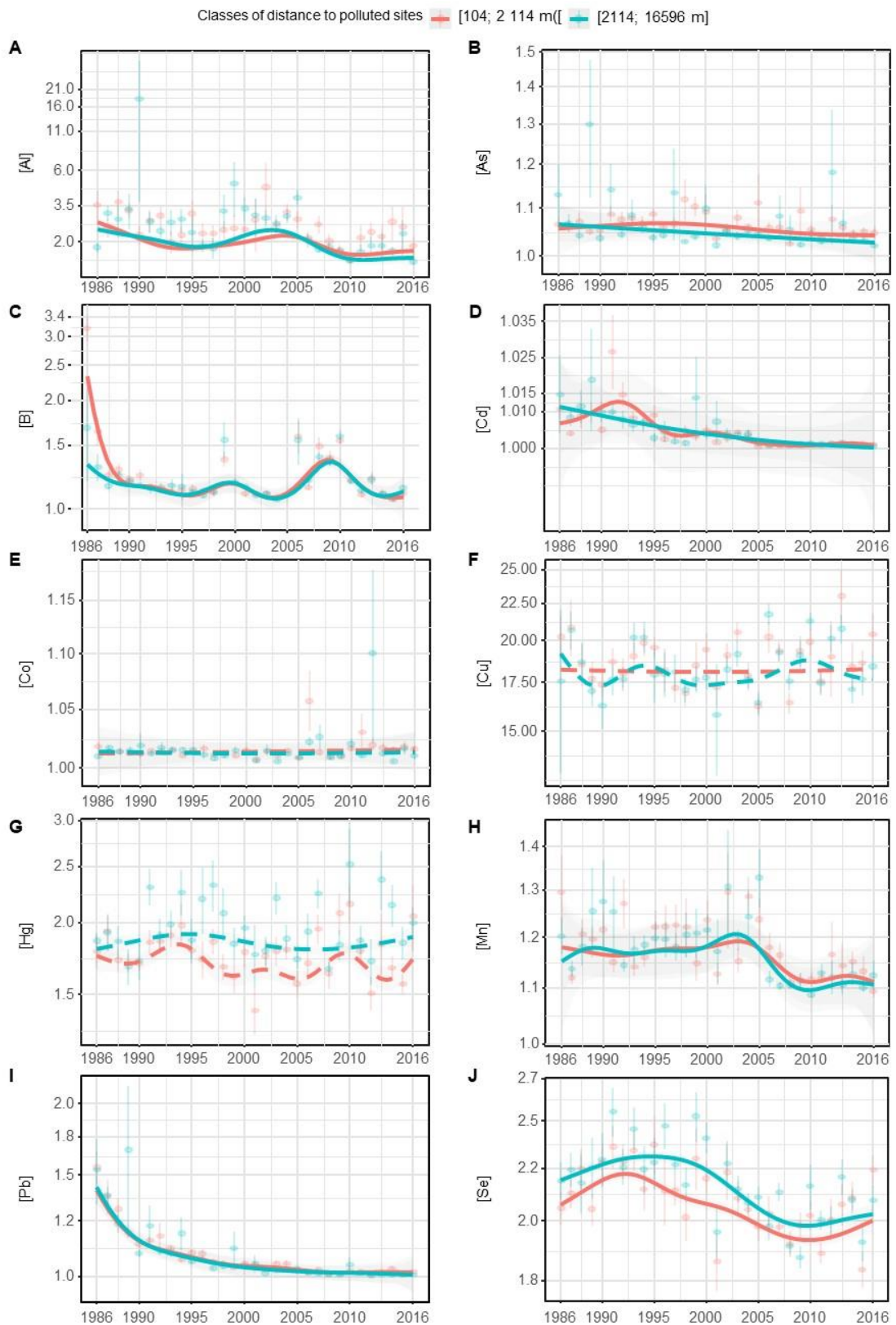
Figure 4. Temporal trends (1986-2016) in the concentrations of toxic elements (Al, As, Cd, Hg, Pb) and essential or beneficial elements (B, Co, Cu, Mn, Se) in tawny owl feathers (in \mu\text{g}\cdot\text{g}^{-1} - average \pm standard error) by class of distance to polluted sites.
