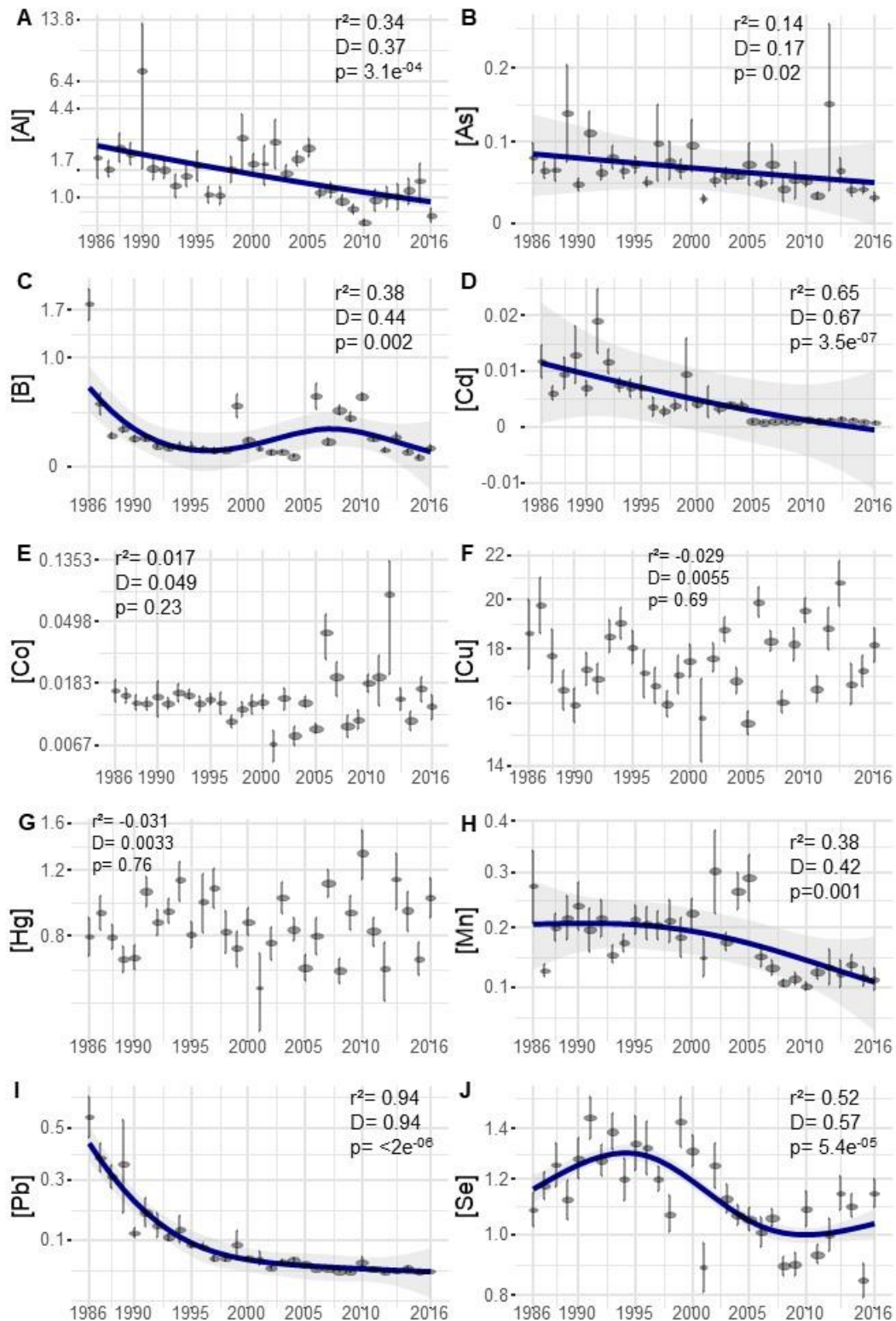
Figure 3. Temporal trends (1986-2016) of toxic elements (Al, As, Cd, Hg, Pb) and essential or beneficial elements (B, Co, Cu, Mn, Se) concentrations in tawny owl feathers ( \mu\text{g}\cdot\text{g}^{-1} ).
