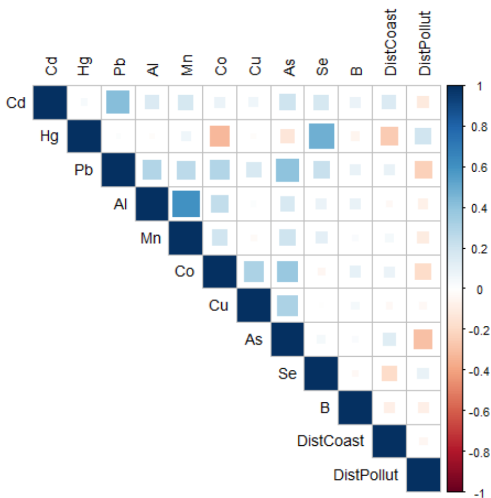
Figure 2. Correlation matrix (Spearman’s rank correlation test) on the dataset gathering metal and metalloid element concentrations ( \mu\text{g}\cdot\text{g}^{-1} ) in owl feathers from 1986 to 2016 and the distance of the nest box where feathers were collected to the coast (“DistCoast”) and to polluted sites (“DistPollut”).
