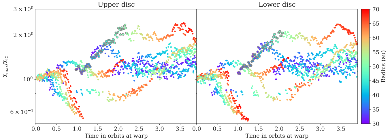
Figure 6. Growth of local dust concentrations throughout the simulation shown in Fig 5. Each point represents a local maximum in the radial dust surface density profile scaled by the initial surface density at that radius. Each point is coloured by its radius, with the uncertainty in the radial measure \pm 1\text{au} . This is shown for the two halves of the disc separately to respect the unique offset ring structure of WInDI. The points circled in grey are associated with the most prominent ring in Fig 5 and used to estimate a growth rate of 1.09 \pm 0.06/\text{orbit} .
