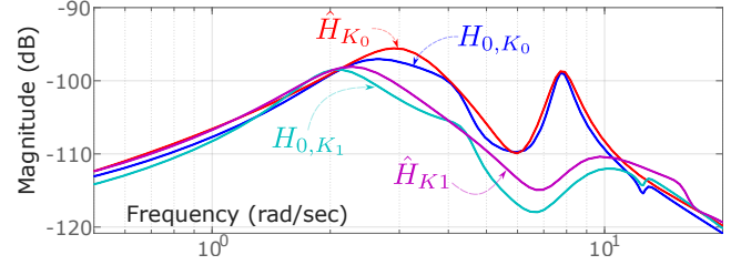
Fig. 8. Assessment of the application of K_{\text{new}} = K_1
