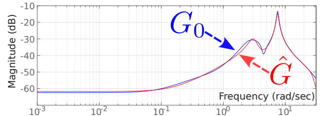
Fig. 7. G_0 and \hat{G} estimated from \hat{T} and K_0 for t=[12.5,17.5] min
