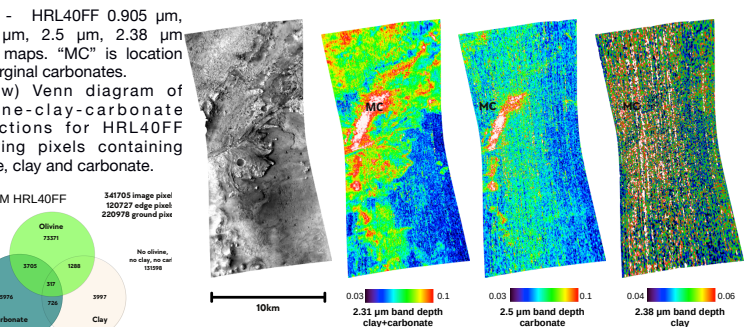
Fig 6 - HRL40FF 0.905 \mu m, 2.31 \mu m, 2.5 \mu m, 2.38 \mu m band maps. "MC" is location of marginal carbonates. (below) Venn diagram of olivine-clay-carbonate detections for HRL40FF showing pixels containing olivine, clay and carbonate.
