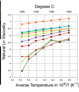
Fig 2. Arrhenius plot of Bottinga-Weill viscosity vs inverse temperature for Maaz (yellow), Séítah (cyan) and Artuby (dark green) compared to terrestrial standards.
