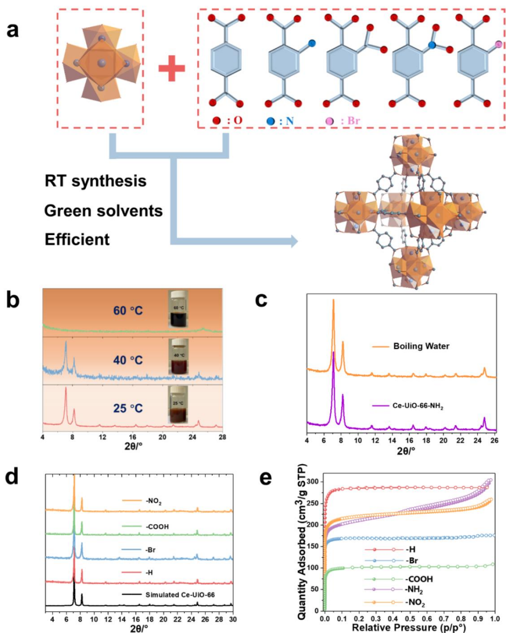
Figure 1. a) Crystal structures of Zr 6 oxo-cluster, linkers, and Ce-UiO-66. b) PXRD ( \lambda_{\text{Cu}}=1.5406\text{\AA} ) patterns of the Ce-UiO-66-NH 2 synthesized at various temperatures (25°C, 40°C, 60°C), insert image: the photography of the resulting solution. c) PXRD patterns ( \lambda_{\text{Cu}}=1.5406\text{\AA} ) of the Ce-UiO-66-NH 2 sample before and after boiling water treatment. d) PXRD patterns ( \lambda_{\text{Cu}}=1.5406\text{\AA} ) of the RT synthesized Ce-UiO-66-X (X= -H, -NO 2 , -COOH, -Br). e) 77K N 2 adsorption-desorption isotherms of the RT synthesized Ce-UiO-66-X.
