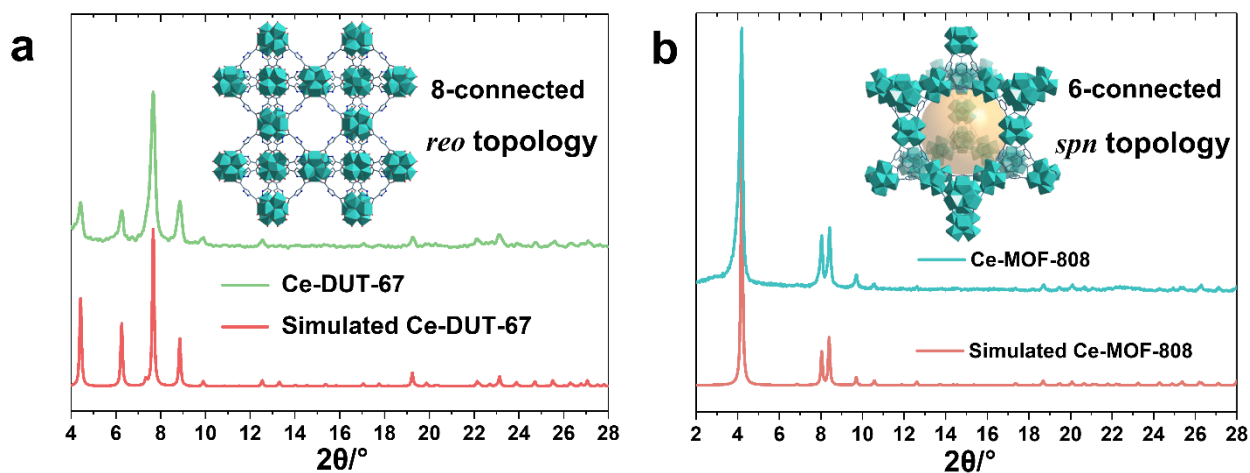
Figure 2. PXRD patterns ( \lambda_{\text{Cu}}=1.5406\text{\AA} ) of synthesized a) 8-connected reo Ce-DUT-67(PDA) and b) 6-connected spn Ce-MOF-808 in comparison to simulated patterns, insert images: structure schemes of the corresponding MOFs.
