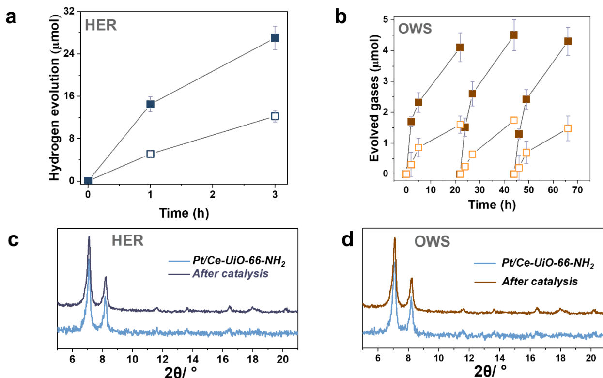
Figure 7. a) Photocatalytic HER using Ce-UiO-66-NH 2 (emptied square) or Pt/Ce-UiO-66-NH 2 (filled square) and, c) the corresponding PXR D pattern of Pt/Ce-UiO-66-NH 2 before and after catalysis. b) Photocatalytic overall water splitting (OWS) into H 2 (filled square) and O 2 (emptied square) using Pt/Ce-UiO-66-NH 2 and, d) the corresponding PXR D patterns of Pt/Ce-UiO-66-NH 2 before and after photocatalytic recycling. Reaction conditions: Photocatalyst amount (20 mg), water (20 mL), simulated sunlight irradiation (150 W Hg-Xe lamp equipped with an AM 1.5G filter), 35 °C.
