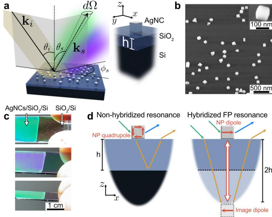
Figure 1. a , BRDF definition schematic. The samples consist of disordered arrays of \sim 100 nm side silver nanocubes (AgNCs) on Si substrates, coated with a thin SiO 2 layer of height h . b , Scanning electron microscope (SEM) image of a typical metasurface with a \sim 8\% surface coverage. A high magnification of a single Ag nanocube is shown in the inset. c , Two-color iridescence is observed for h \approx 640 nm under sunlight illumination for various viewing \theta and lighting \theta_i directions. The photographs are extracted from the Supplementary Movie 1. Half of the sample surface is not covered by nanocubes; it does not scatter light and appears dark when the viewing direction differs from the specular reflection direction. d , The iridescence is due to two types of resonance modes with markedly different physical properties documented in Supplementary Note 3.
