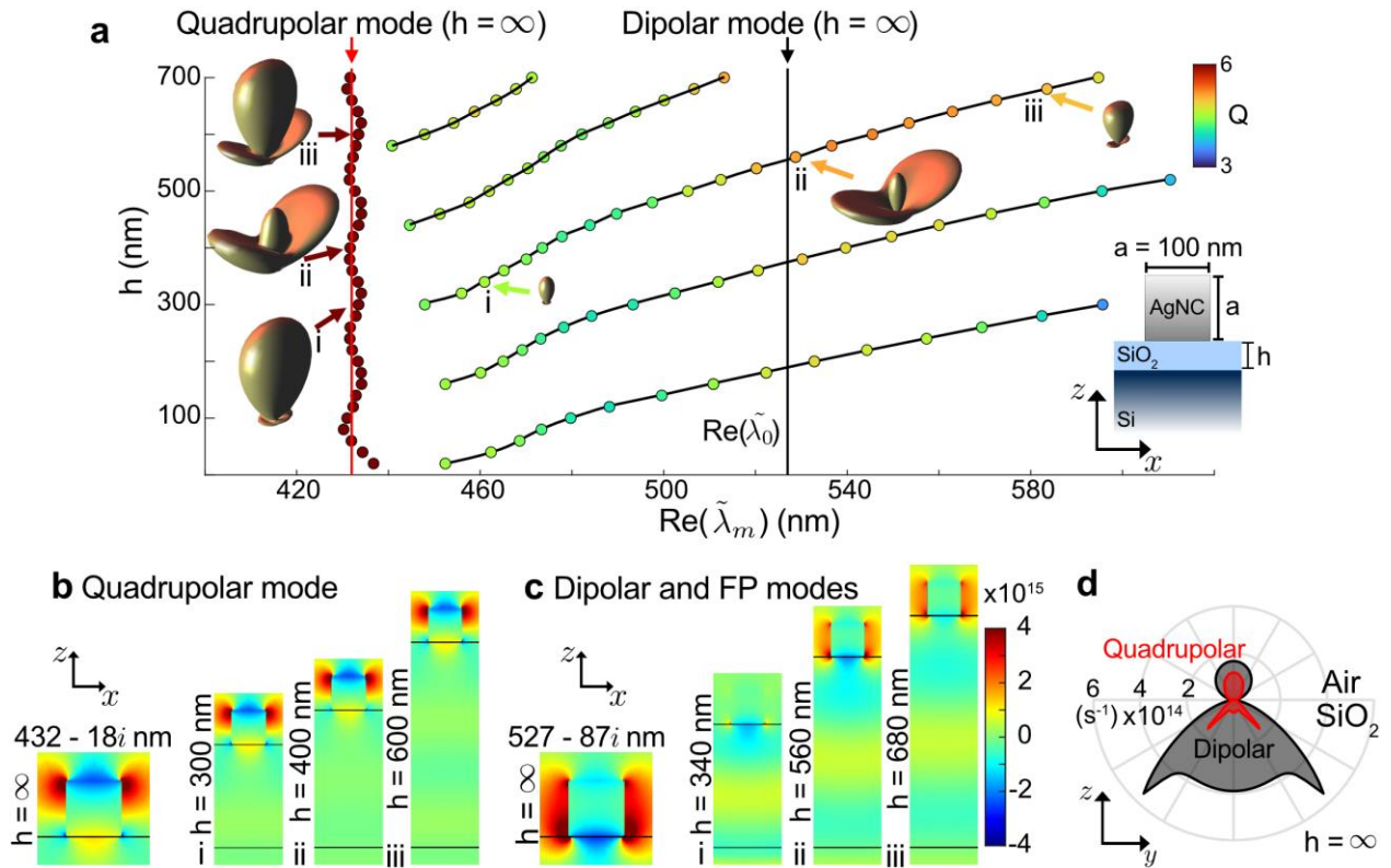
Figure 3. a, Eigenwavelengths of the dominant QNMs for a (100×100×100 nm 3 ) Ag nanocube on a Si substrate coated with a silica film of thickness h . The color of the dots represents the quality factor Q . The scattering diagrams of several normalized QNMs are also displayed in the insets. The solid vertical lines correspond to the real part of the eigenwavelengths of the electric dipolar (ED) (black) and quadrupolar (EQ) (red) modes of the same nanocube on a SiO 2 substrate ( h = \infty ). b-c, Near-field distributions of the quadrupolar (b) and dipolar (c) modes for three values of h labeled as i, ii and iii in a. The maps show the real part of the QNM electric field x -component, \tilde{E}_x , in the xz -plane. The fields are computed and normalized with the freeware MAN. 47 d, Scattering diagrams of the normalized dipolar and quadrupolar QNMs for h = \infty .
