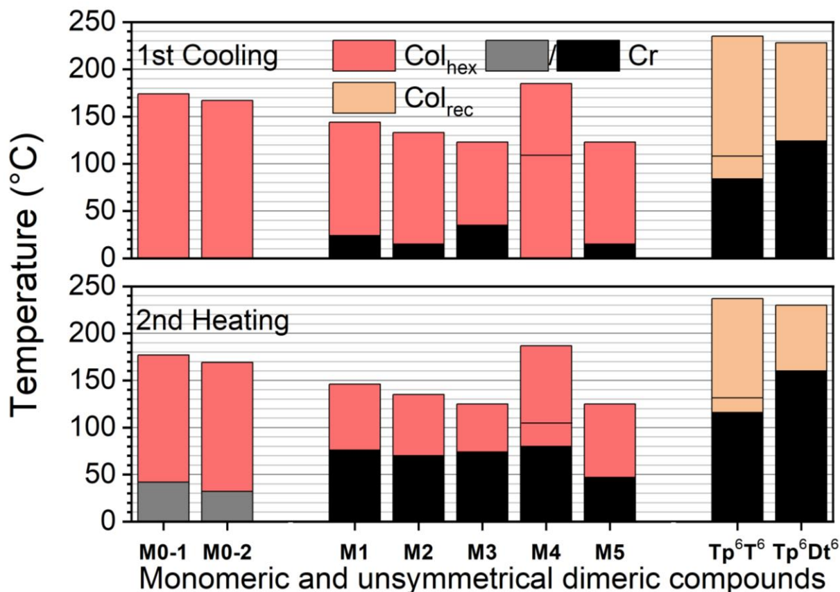
Figure 1. Phase diagrams (top: 1st cooling; bottom: 2nd heating) of the precursors, monomeric and unsymmetrical dimeric DLCs. For M4 , a transition between two Col hex mesophases was detected by DSC and POM; For Tp 6 T 6 , a transition between two rectangular phases was detected by DSC and SWAXS.
