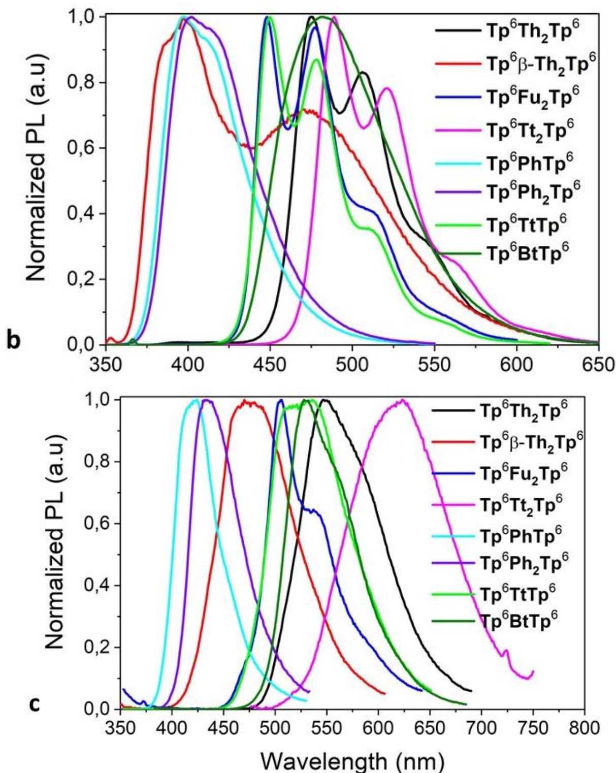
Figure 8. (a) UV-Vis absorption spectra, (b) fluorescence emission spectra in solution, and (c) thin film fluorescence emission spectra of various \pi -bridged dimers.
