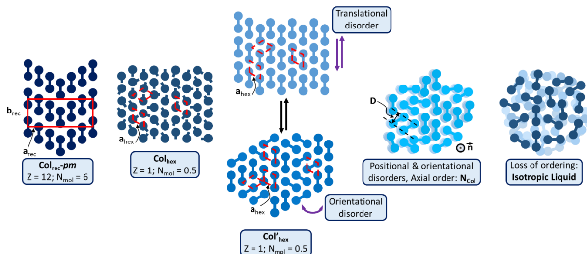
Figure 6. Schematic representation of the various supramolecular mesomorphous arrangements induced by the \pi -bridged dimeric mesogens: the Col_{rec}^{pm} phase with chevron arrangements of the TP dimers; Col_{hex} phase, differentiated by translational or orientational order fluctuations; the Col_{hex} phase of Tp^{\beta}Th_2Tp^{\beta} is similar to that of the monomeric precursors (Fig. S68, ESIf); the N_{Col} phase characterized by loss of positional and orientational orders, but with short-range columns aligned along one main direction (axial order), the director \vec{n} ; isotropic liquid: no persisting molecular ordering.
