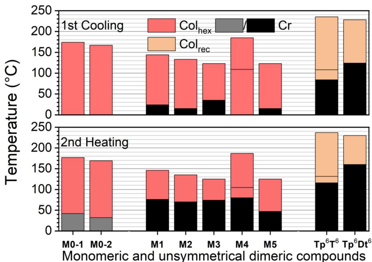
Figure 1. Phase diagrams (top: 1st cooling; bottom: 2nd heating) of the precursors, monomeric and unsymmetrical dimeric DLCs. For M4 , a transition between two \text{Col}_{\text{hex}} mesophases was detected by DSC and POM; For Tp 6 T 6 , a transition between two rectangular phases was detected by DSC and SWAXS.
