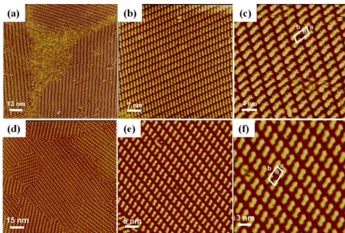
Figure 7. Large-scale (a), medium range (b) and high-resolution (c) STM images of the self-assembly structure of Tp 6 Tt 2 Tp 6 on the 1-phenyloctane/HOPG interface (imaging parameters: (a): I_{\text{set}} = 299.1 pA, V_{\text{bias}} = 699.8 mV; (b): I_{\text{set}} = 247.2 pA, V_{\text{bias}} = 847.2 mV; and (c): I_{\text{set}} = 299.1 pA, V_{\text{bias}} = 699.8 mV); large-scale (d), medium range (e) and high-resolution (f) STM images of the self-assembly structure of Tp 8 Th 2 Tp 8 on the 1-phenyloctane/HOPG interface (imaging parameters: (d): I_{\text{set}} = 271.6 pA, V_{\text{bis}} = 770.0 mV; (e): I_{\text{set}} = 271.6 pA, V_{\text{bis}} = 770.0 mV; and (f): I_{\text{set}} = 271.6 pA, V_{\text{bis}} = 770.0 mV).
