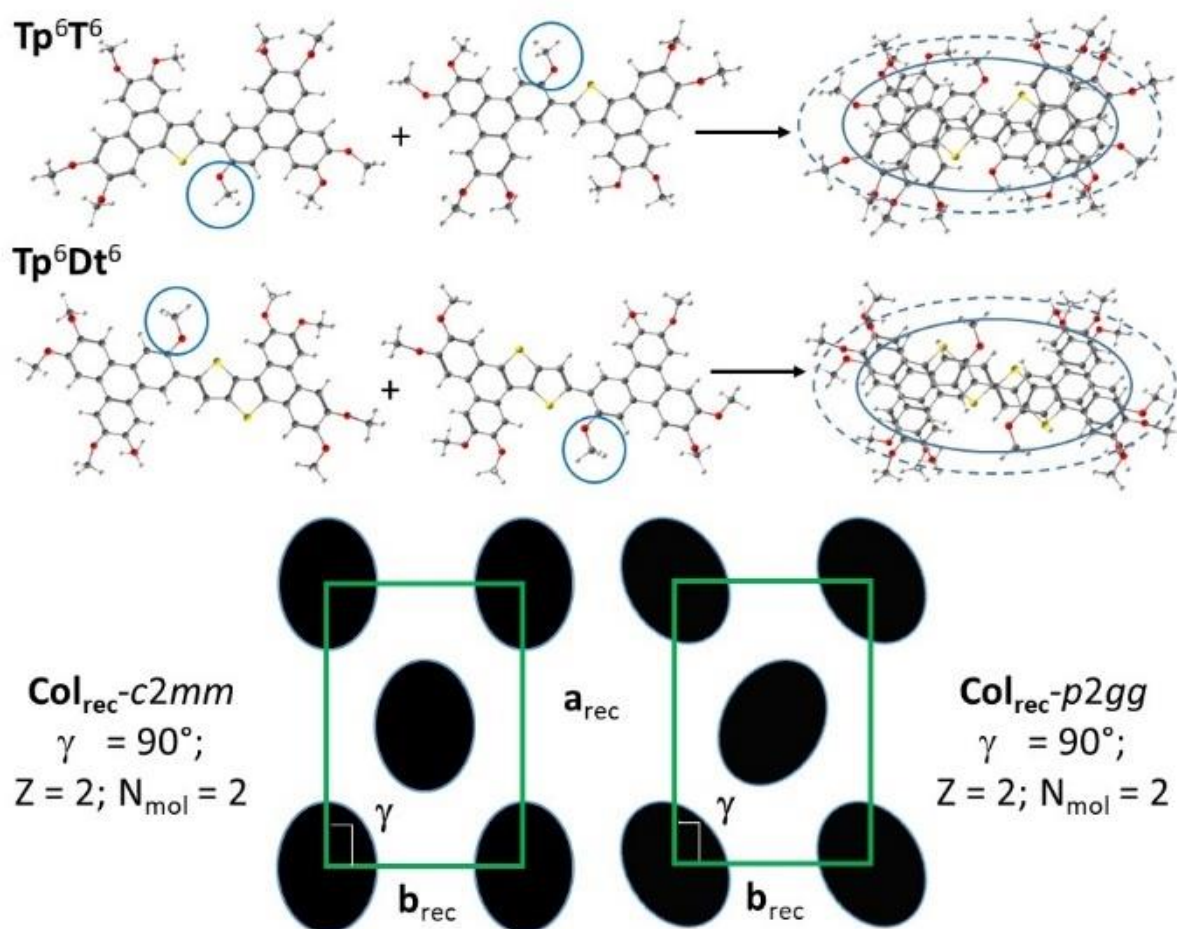
Figure 2. Schematic representations of molecular self-assemblies and supramolecular organizations in the various mesophases of the unsymmetrical \sigma -dimers, Tp 6 T 6 ( c2mm and p2gg ) and Tp 6 Dt 6 ( c2mm ); a_{\text{rec}} , b_{\text{rec}} , \gamma : lattice parameters and angle, Z : number of columns per lattice and N_{\text{mol}} : number of mesogens per lattice; the central chain is circled in blue (the chains are not represented for clarity).
