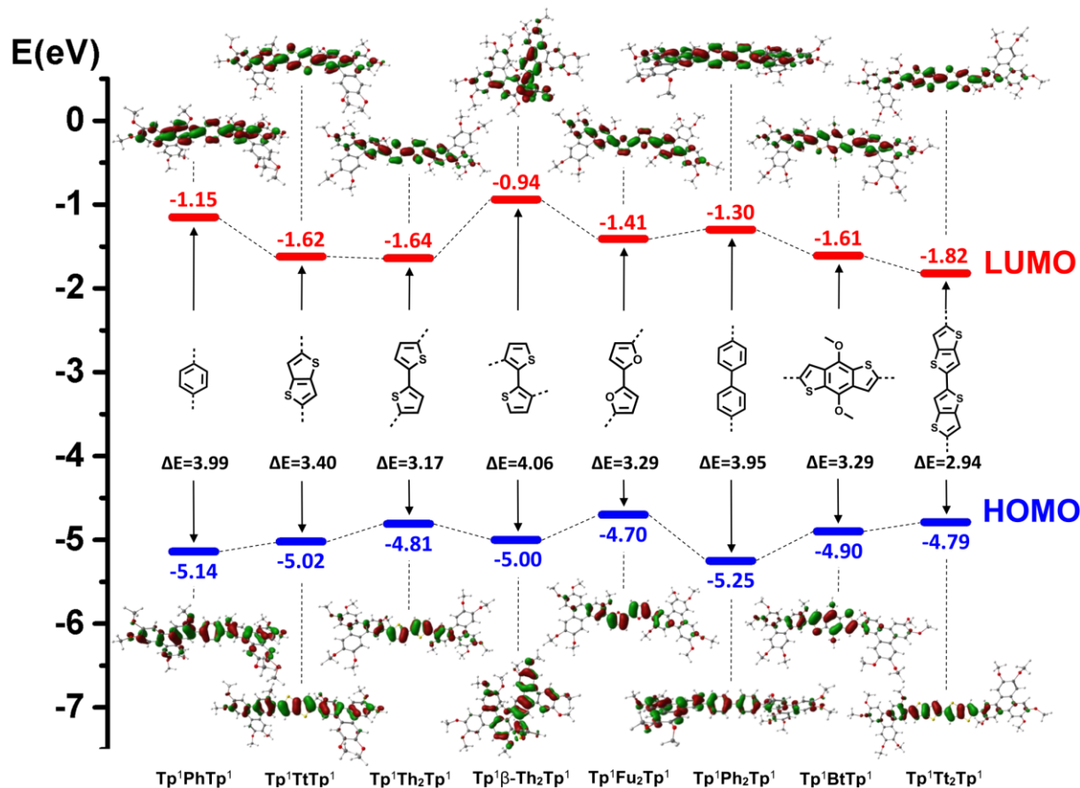
Figure 9. HOMO–LUMO and energy gaps of the discotic dimers.
