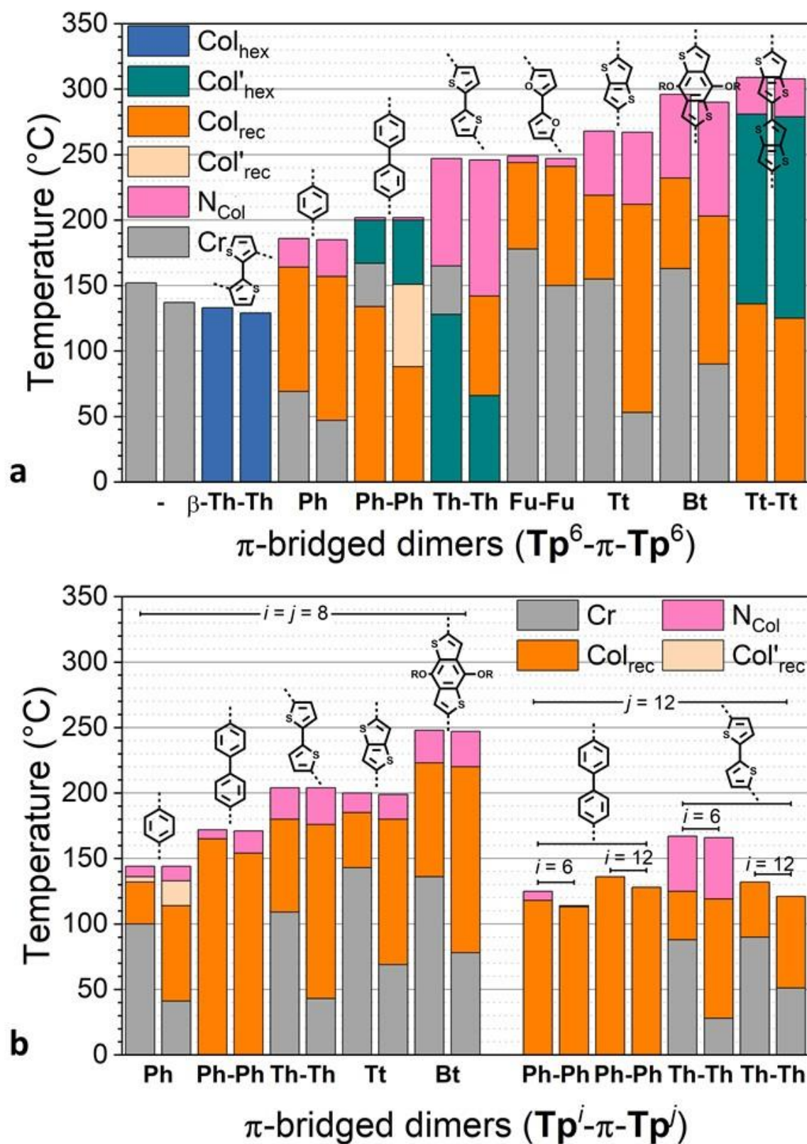
Figure 3. Phase diagram of \pi -bridged discotic dimers (both 2nd heating and 1st cooling are displayed in bar diagram for each compound): (a) \text{Tp}^6\text{-}\pi\text{-Tp}^6 and (b) \text{Tp}^i\text{-}\pi\text{-Tp}^j ( i, j = 6, 8, 12 ).
