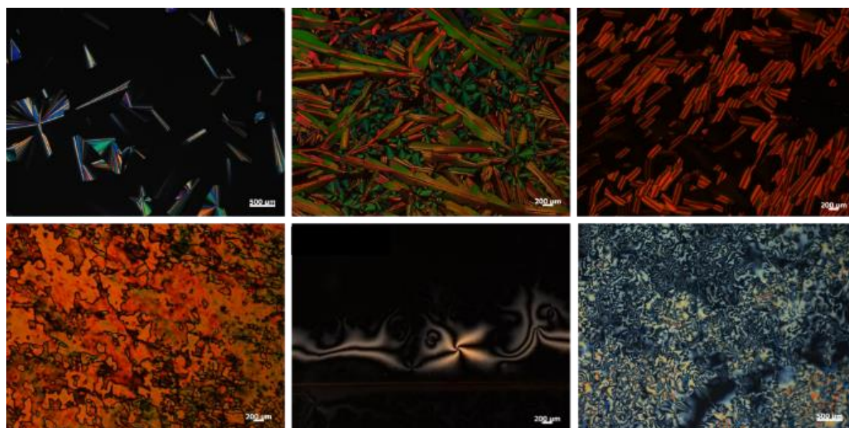
Figure 4. Selected POM textures of some representative \pi -bridged dimers. Top row: Tp 6 β-Th 2 Tp 6 (100 °C, Col hex ), Tp 6 Fu 2 Tp 6 (228 °C, Col rec ), and Tp 6 TtTp 6 (178 °C, Col hex ); bottom row: N Col of Tp 8 Th 2 Tp 8 (195 °C), Tp 6 Ph 2 Tp 6 (174 °C), and Tp 8 Ph 2 Tp 8 (165 °C). Additional textures can be found in Fig. S57 (ESI†).
