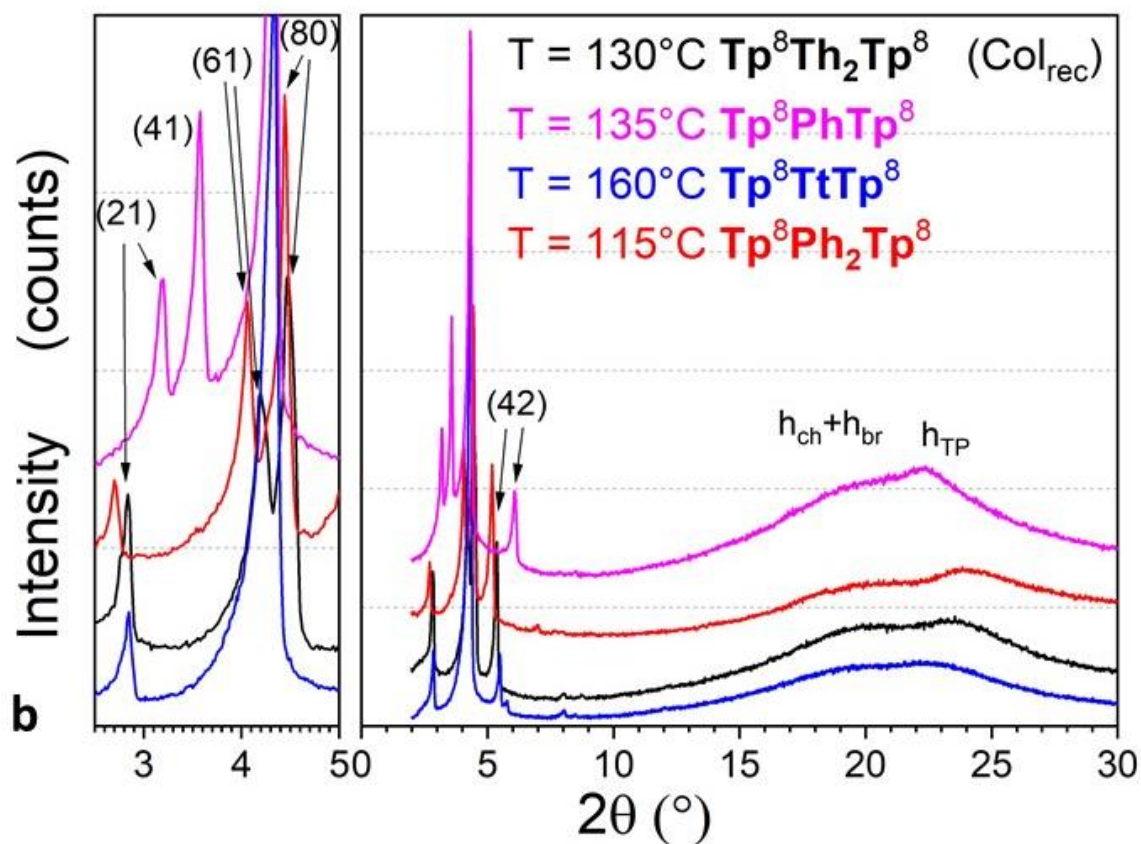
Figure 5. Representative SWAXS patterns of some representative dimeric compounds \text{Tp}^i\text{-}\pi\text{-Tp}^j ( i, j = 6, 8 ) recorded at various temperatures in (a) \text{Col}_{\text{hex}} ( \text{Tp}^6\text{-}\pi\text{-Tp}^6 , top) and (b) \text{Col}_{\text{rec}} ( \text{Tp}^8\text{-}\pi\text{-Tp}^8 , bottom)
