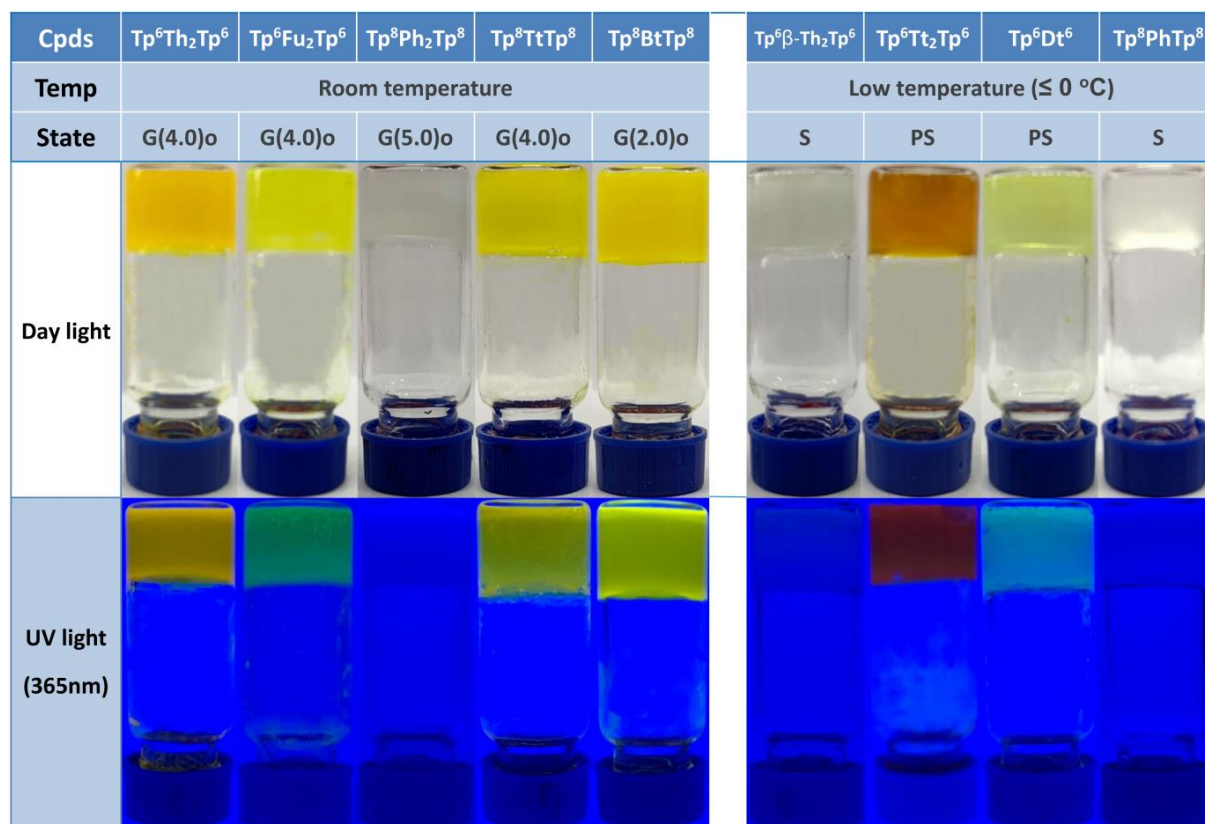
Figure 10. Gels and frozen solutions of the dimers formed in cyclohexane on slow cooling, at room temperature and below 0\text{ }^\circ\text{C} , in day light (top) and under UV irradiation (365 nm, bottom). G, S and PS indicate the state of the mixture corresponding to gel, solution and poor solution, respectively. The numbers in brackets correspond to the critical (minimum) gelation concentration (CGC/MGC) in \text{mg mL}^{-1} ; “o” indicates that the gel is opaque.
