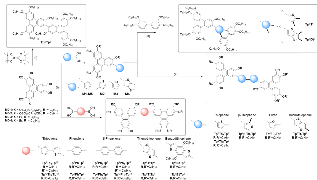
Scheme 1. General synthetic scheme and nomenclature of the various monomeric and dimeric compounds (displayed in the frames): (i) Suzuki coupling; (ii) Scholl oxidative cyclodehydrogenation; and (iii) annulative \pi -extension (APEX) reactions. Nomenclature: Tp ij - \pi -Tp ij , where Tp ij is the triphenylene moiety substituted by 5 alkoxy chains, \text{OC}_n\text{H}_{2n+1} , of length n = i and/or j , with i, j = 6, 8, 12 , and \pi for the rigid, conjugated bridge: \pi = \text{Th}, \text{Th}_2 for (bi)thiophene-, Fu, Fu 2 for (bi)furan-, Tt, Tt 2 for (bi)thienothiophene-, Ph, Ph 2 for (bi)phenylene-, and Bt for benzodithiophene-based bridge.
