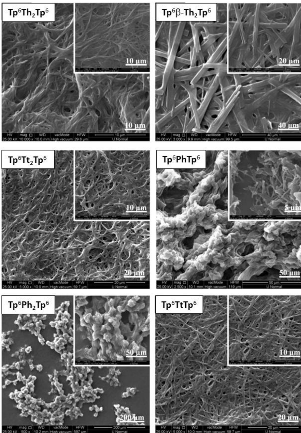
Figure 11 Self-assembled morphologies of some representative \pi -bridged dimers: SEM images of xerogels or solution-deposited micro-particles from organic solvents.
