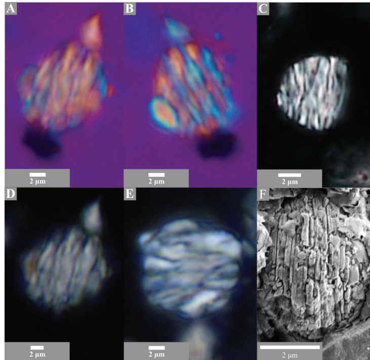
Fig. 4. Prinsiosphaera triassica crenulata (Jafar 1983) in LM (A – E) with XPL and gypsum plate (A, B) and under the SEM (F). Specimens show calcite lamellae organized in stripes and are from the middle Rhaetian, corresponding to sample ZL 52.8554.
