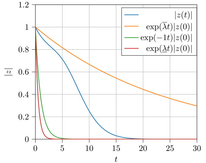
Fig. 2. Evolution of the norm of z(t) , and its upper bound evolution through the explicit value of the convergence rate -\bar{\lambda} , orange curve. While its evolution is lower bounded by the exponential function with convergence rate -\underline{\lambda} , in red. Moreover, see that the exponential function with convergence rate given by the associated eigenvalue \lambda = -1 does not give any particular information.
