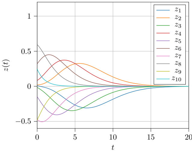
Fig. 1. Evolution of the components of the z(t) state, whose dynamics is associated to the eigenvalue \lambda = -1 with geometric multiplicity g = 10 , initialized at z(0) = z_0 .
