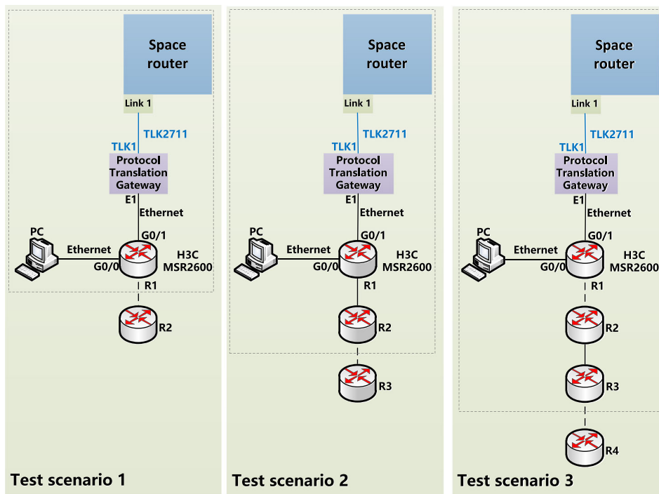
FIGURE 16 Route computation time experiment setup.
