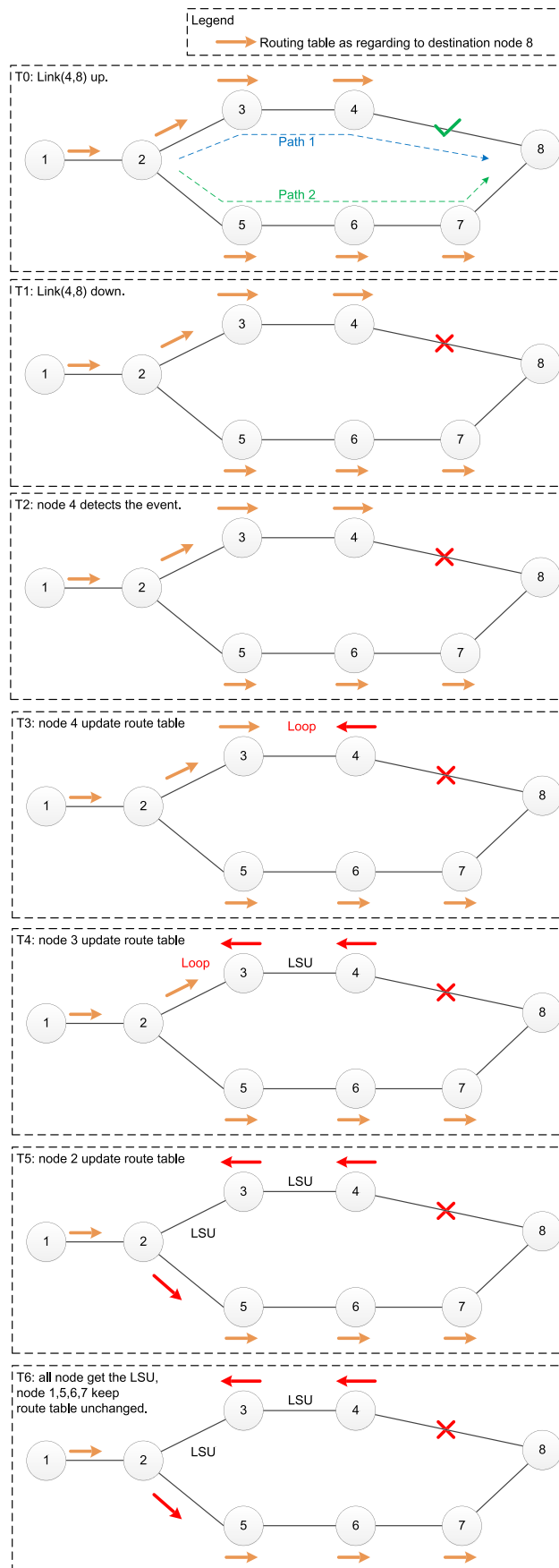
FIGURE 5 The response process of OSPF after the link is down.
