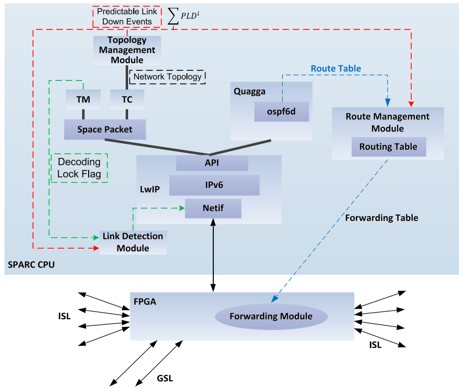
FIGURE 11 Space router architecture.
