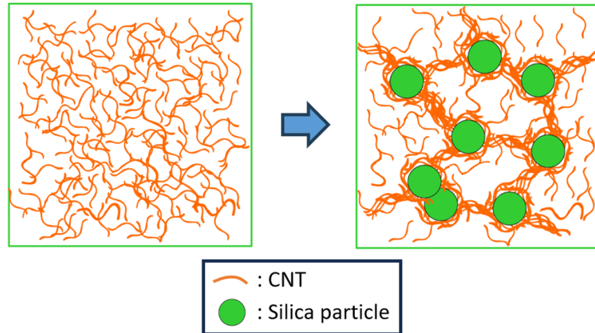
Figure 4. Illustration of CNT network morphology change with the inclusion of silica MPS in CNT- PDMS composites. CNTs are closely bound on the surface of silica particles with PDMS as a binder. CNT bundles connect the sub-networks like a bridge between neighboring silica particles to complete transport pathways throughout the sample.
