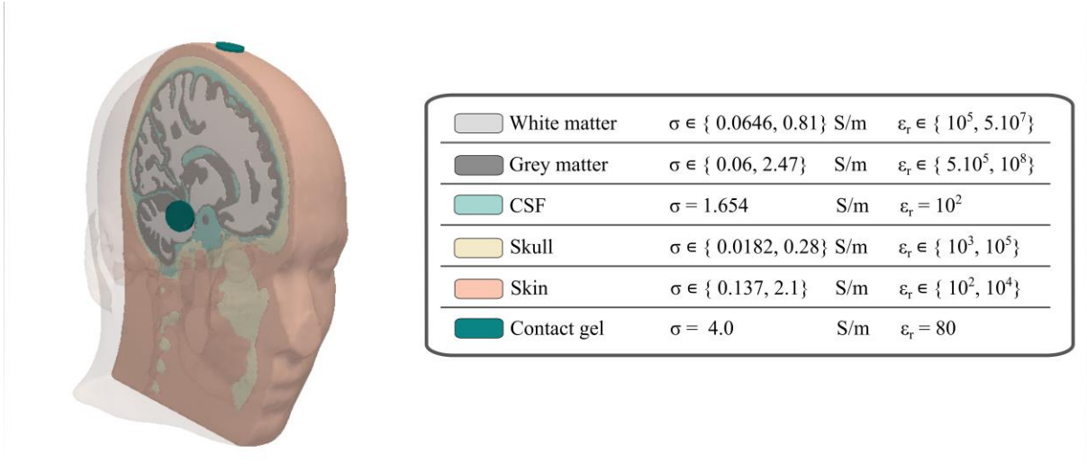
Figure 1: Problem formulation. Head model geometry with the five main tissues (left) and associated dielectric properties values (right).
