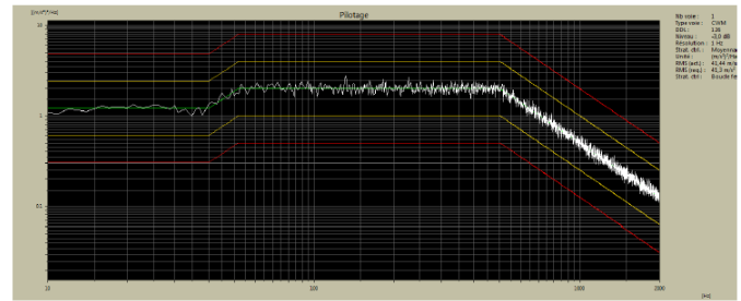
Fig. 6. Vibration power density for IEC 60068-2-64
