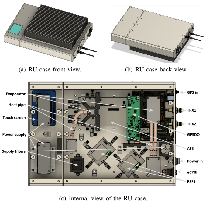
Fig. 2. RU fan-less case front/back (a)-(b) and internal views (c)
