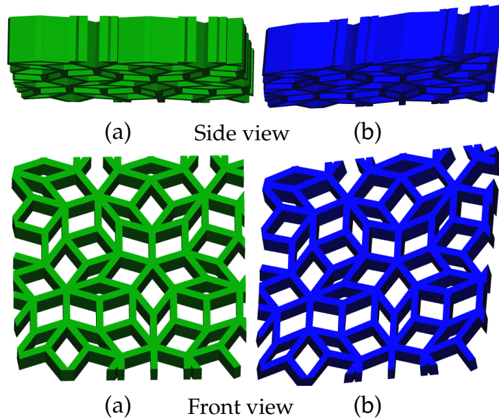
FIGURE 4 – (a) The Initial CAD model (b) the deformed geometry that we try to recover.
