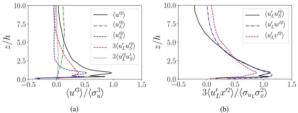
FIGURE 6 – (a) : skewness decomposition of the streamwise velocity \langle u'^3 \rangle in small-scale skewness \langle u'_S{}^3 \rangle , large-scale skewness \langle u'_L{}^3 \rangle , and cross-terms 3\langle u'_L u'_S{}^2 \rangle and 3\langle u'_L{}^2 u'_S \rangle . (b) : non-linear cross-terms of the skewness decomposition, \langle u'_L u'_S{}^2 \rangle (black line), \langle u'_L v'^2 \rangle (red dashed line) and \langle u'_L w'^2 \rangle (blue dashed-dotted line). All components are spatially and temporally averaged, and normalized by \langle \sigma_u^3 \rangle (a), or \langle \sigma_{u_L} \sigma_x^2 \rangle (b).
