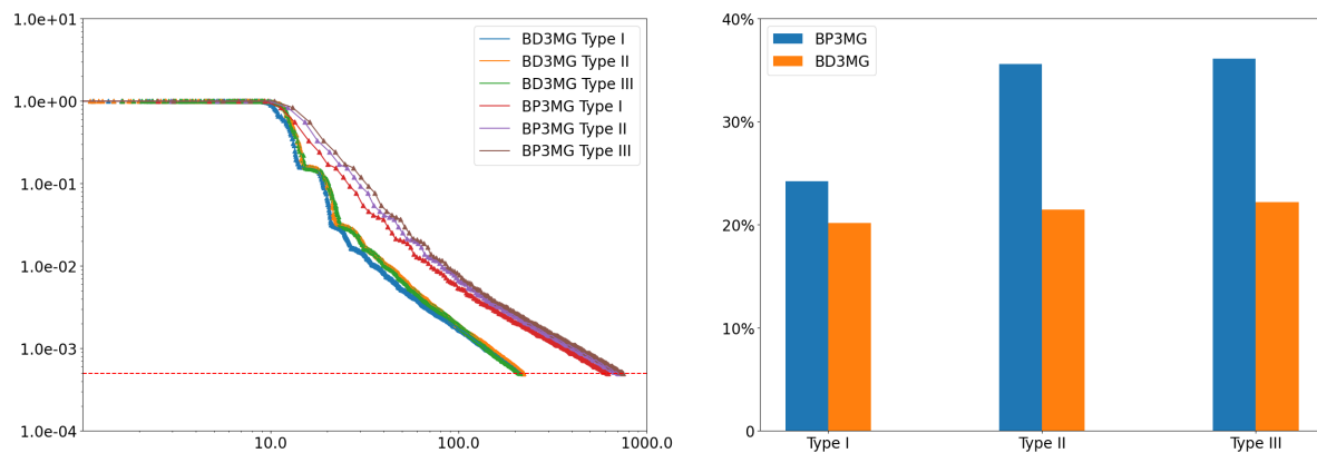
Figure 4: Numerical comparisons between BD3MG and BP3MG for FlyBrain restoration under imbalanced computing power: evolution of the relative increment \|x^{k+1} - x^k\| / \|x^k\| along time (in sec.) for each of the three experimental settings in log-log scale (left), and averaged ratio of workers CPU idle time over the entire optimization process for each scenario (right).
