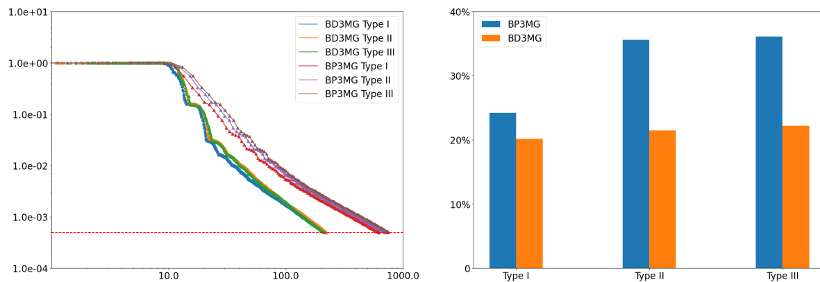
Figure 4: Numerical comparisons between BD3MG and BP3MG for FlyBrain restoration under imbalanced computing power: evolution of the relative increment \|\mathbf{x}^{k+1} - \mathbf{x}^k\| / \|\mathbf{x}^k\| along time (in sec.) for each of the three experimental settings in log-log scale (left), and averaged ratio of workers CPU idle time over the entire optimization process for each scenario (right).
