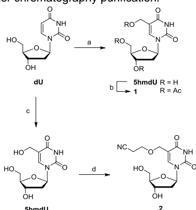
Scheme 1. Reagents and conditions: a) 37% HCHO (20 eq), Et 3 N (13 eq), H 2 O, 3 days 80°C; b) Ac 2 O, pyridine, DMAP, 16h, r.t., 77% (two steps); c) (HCHO) n in 5M KOH, 90°C, 3 days, 67% d) Amberlyst 15 (1g/mmol 5hmdU), cyanoethanol (5 eq), MeCN, r.t., 90%.
