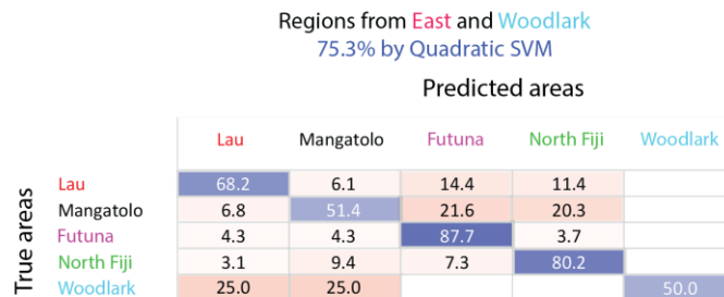
Figure 5: Confusion matrices of the classification of Shinkailepas tollmanni encapsulated larvae based on shell geochemistry at the region scale. a: Using Mn and Ba as predictors for sites sampled in the Manus and Woodlark areas only (western region). b: Using Mg, Mn, Fe, Zn, Sr, Ba and Pb as predictors for sites from Woodlark, North Fiji, Futuna, Lau, and Mangatolo areas (eastern region and Woodlark). c: Using Mg, Mn, Fe, Zn, Sr, Ba and Pb as predictors for all areas except Manus (eastern region and Woodlark). For each line, corresponding to one site (a, c) or one area (b), percentage of correct classification are indicated in blue and wrong classification in red.
