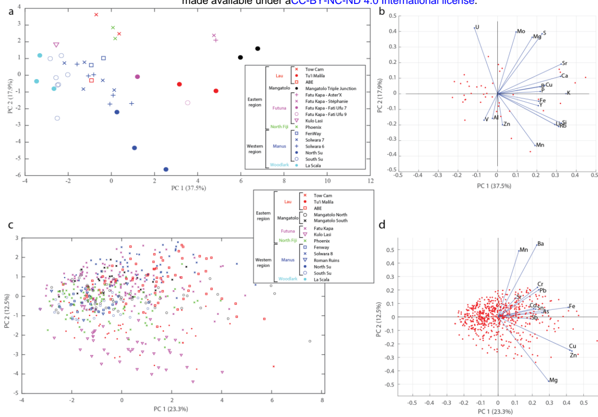
580 Figure 3: Principal Component Analysis of Ifremeria habitat water compositions (a-b) and Shinkailepas tollmanni larval shell compositions (c-d) between sites, showing principal components 1 and 2. The legend gathers all sites by area (Lau, Mangatolo, Futuna, North Fiji, Manus and Woodlark) and by region (East and West). The variance explained by each principal component is given in parentheses (55.4% and 35.8% on the first two axes for habitat water and S. tollmanni larval shells, respectively).
