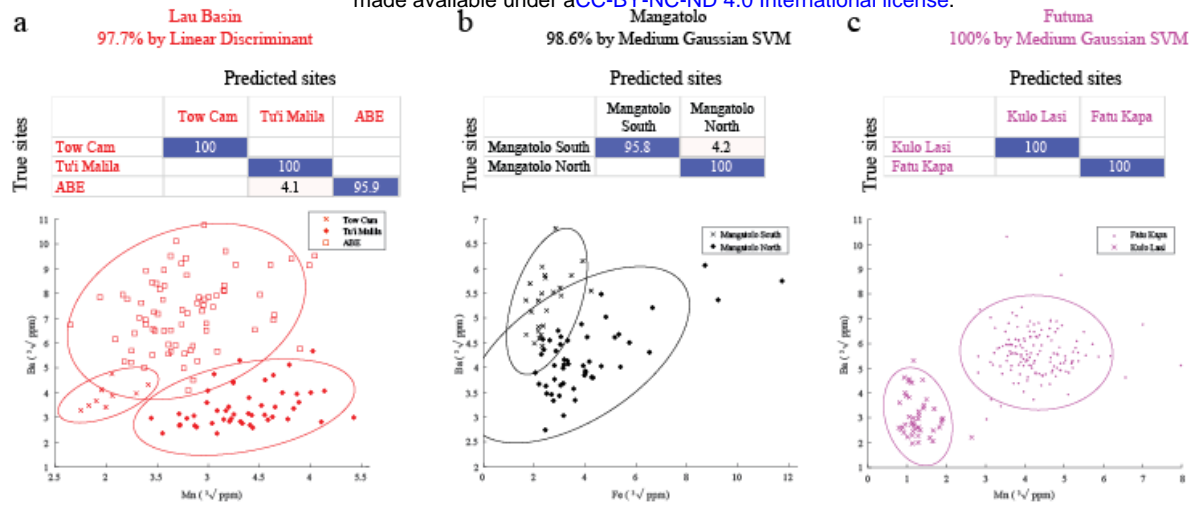
595 Figure 6: Confusion matrices of the classification of Shinkailepas tollmanni encapsulated larvae based on shell geochemistry between sites for each eastern area and scatter plots of corresponding datasets (a: Lau; b: Mangatolo; c: Futuna volcanic arc). For each line of the matrices (corresponding to one site), percentage of correct classification are indicated in blue and wrong classification in red. For each matrix, the precision and type of model are indicated. The elements kept to build these models are Mn and Ba for Lau Basin and Futuna volcanic arc, and Fe and Ba for Mangatolo, as illustrated by the scatter plots.
