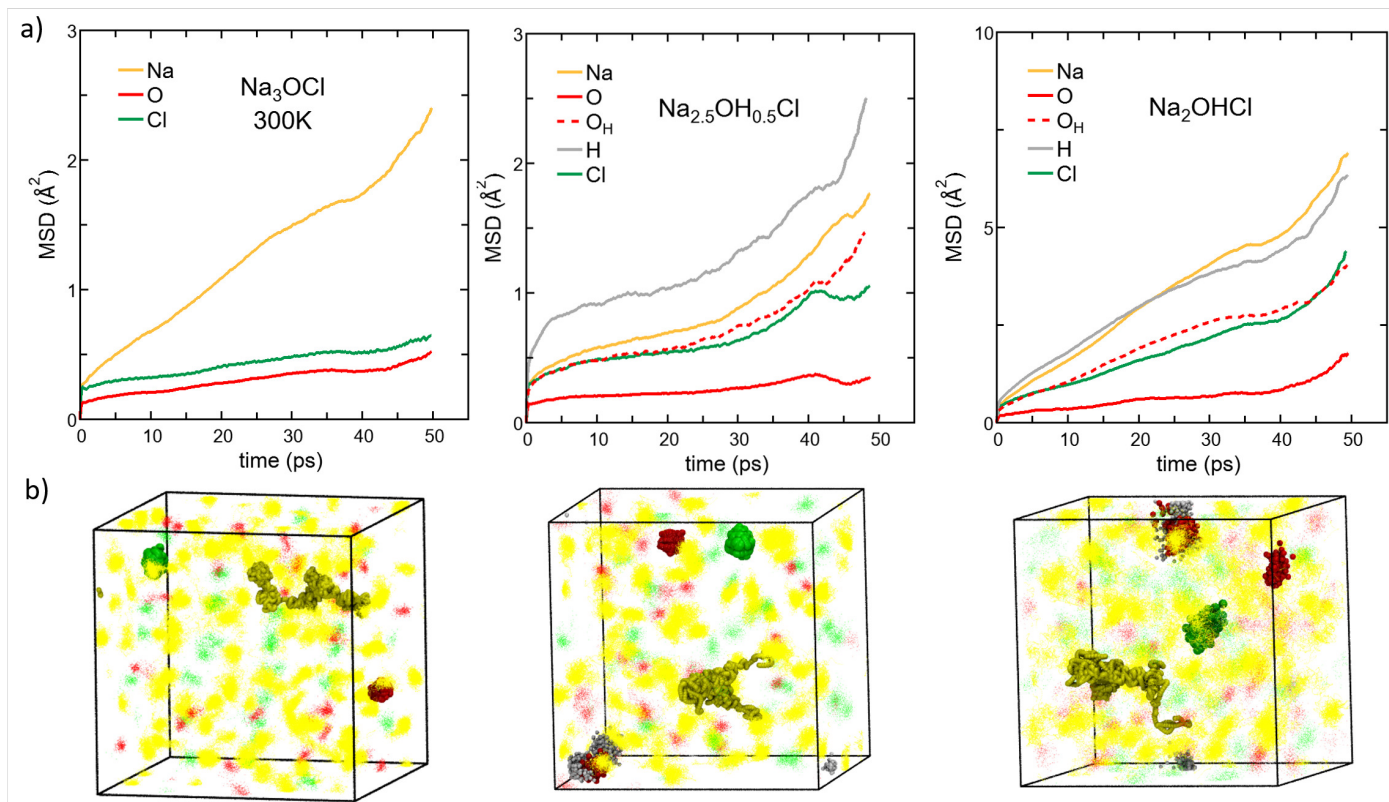
Fig. 8 (Color online) a) MSD versus time for each element in amorphous \text{Na}_{3-x}\text{OH}_x\text{Cl} ( x = 0, x = 0.5, x = 1 ) at T = 300 K. Colors legend: Na, yellow; O non-bonded to H atoms, red (solid line); O bonded to H atoms, red (dashed line); H, grey; Cl, green. Note that the MSD calculated at the temperatures T = 300 K, T = 450 K, T = 600 K, T = 800 K, T = 1000 K are reported in the ESI, (Fig. S1). b) Density plots \sim 50 ps trajectories of all elements are shown as dots for the three models simulated at 300 K. Na, O, and Cl atoms positions are given in yellow, red, and green, respectively. H atoms are omitted for clarity. Examples of an individual local Na migration path and Cl, O and OH local vibrations are highlighted in spheres.
