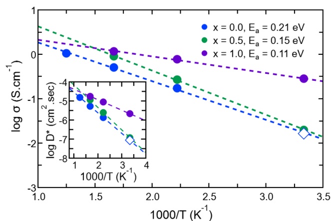
Fig. 12 (Color online) Na-ion self-diffusion coefficients (inset) and conductivities of amorphous \text{Na}_{3-x}\text{OH}_x\text{Cl} ( x = 0, x=0.5, x=1 ). We also report the activation energies of Na ionic conduction obtained via a linear Arrhenius fit. Closed circles correspond to FPMD data and open circles correspond to data at T = 300\text{ K} extrapolated by using the linear Arrhenius fit.
