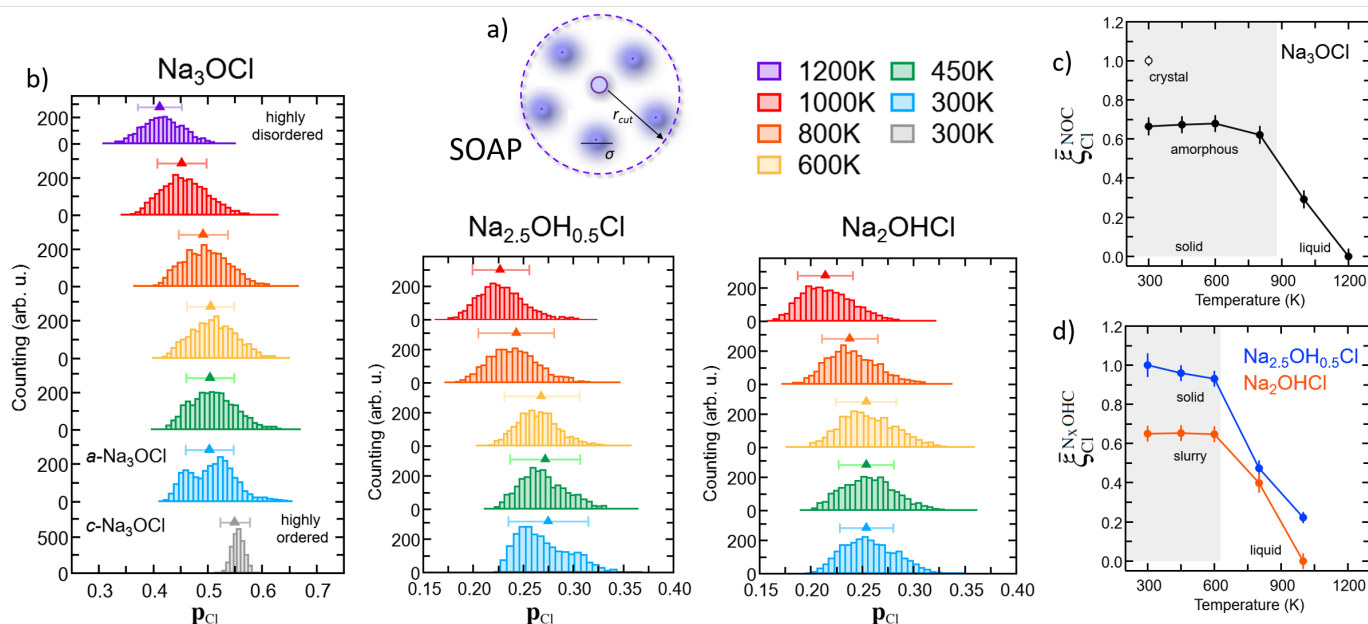
Fig. 7 (Color online) a) Schematic representation of the SOAP descriptor. b) \text{Na}_3\text{OCl} , \text{Na}_{2.5}\text{OH}_{0.5}\text{Cl} , and \text{Na}_2\text{OHCl} SOAP p_{\text{Cl}} distributions computed at different temperatures. The data computed for crystalline \text{Na}_3\text{OCl} is also reported. Structural disorder degree of the three models framed as SOAP similarity to crystalline \text{Na}_3\text{OCl} ( \xi_{\text{Cl}}^{\text{NOC}} , c)) and to amorphous \text{Na}_{2.5}\text{OH}_{0.5}\text{Cl} phase ( \xi_{\text{Cl}}^{\text{N}_x\text{OHC}} , d)), respectively.
