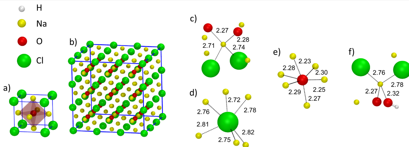
Fig. 5 (Color online) a) Representation of the unit cell of crystalline \text{Na}_3\text{OCl} . The red polyhedra identify the octahedron O site. b) Crystalline supercell of 135 atoms (unit cell replicated 3 \times 3 \times 3 ). c-e) Coordination units for Na, O, and Cl found in amorphous \text{Na}_3\text{OCl} at T = 300 K: a fourfold Na atom ( \text{O}_2\text{Cl}_2 ) (c), a sixfold Cl atom (d), a sixfold O atom (e). f) A Na atom found in amorphous \text{Na}_{2.5}\text{OH}_{0.5}\text{Cl} coordinated by at least an O atom as a hydroxyl group. Counter-ions interatomic bonds are identified by a dashed line with the corresponding values. We show the atoms within a radial cutoff of 3.3 Å. Color legend: Na, yellow; O, red; Cl, green; H, white.
