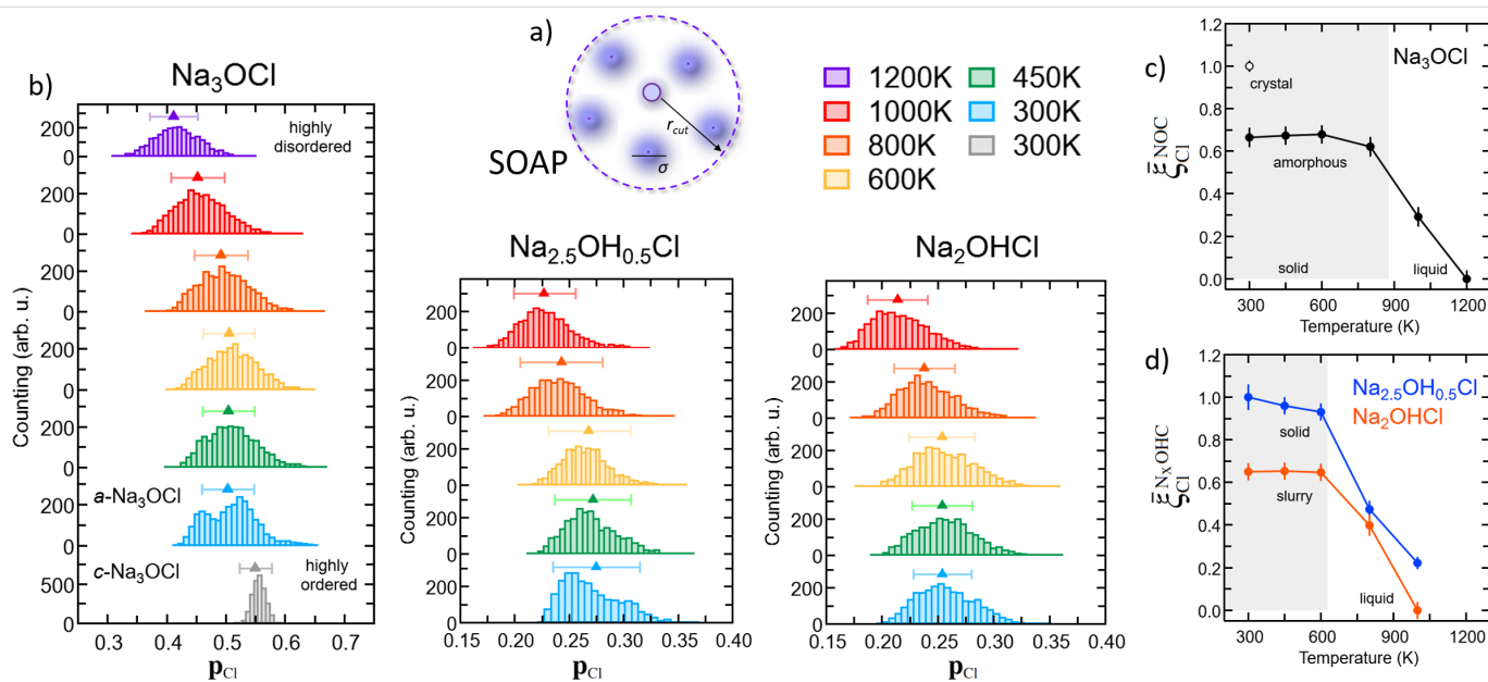
Fig. 7 (Color online) a) Schematic representation of the SOAP descriptor. b) \text{Na}_3\text{OCl} , \text{Na}_{2.5}\text{OH}_{0.5}\text{Cl} , and \text{Na}_2\text{OHCl} SOAP \bar{p}_{\text{Cl}} distributions computed at different temperatures. The data computed for crystalline \text{Na}_3\text{OCl} is also reported. Structural disorder degree of the three models framed as SOAP similarity to crystalline \text{Na}_3\text{OCl} ( \bar{\xi}_{\text{Cl}}^{\text{NOC}} , c)) and to amorphous \text{Na}_{2.5}\text{OH}_{0.5}\text{Cl} phase ( \bar{\xi}_{\text{Cl}}^{\text{N}_{2.5}\text{OHC}} , d)), respectively.
