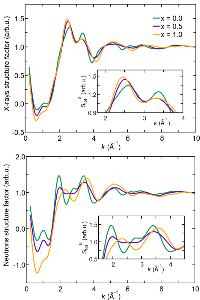
Fig. 2 (Color online) Total X-rays (top) and neutrons (bottom) structure factors for amorphous \text{Na}_{3-x}\text{OH}_x\text{Cl} ( x=0, x=0.5, x=1 ) obtained through Fourier transform (FFT) of the total pair correlation functions at T=300 K. Insets: zoom-in in the 1.8\text{--}4.0 \text{ \AA}^{-1} and 1.5\text{--}4.5 \text{ \AA}^{-1} ranges, respectively.
