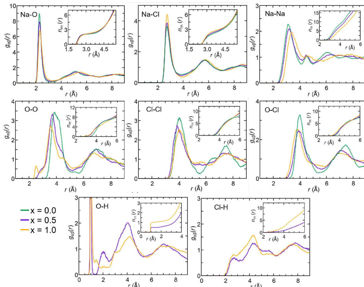
Fig. 4 (Color online) Partial pair correlation functions g_{\alpha\beta}(r) for amorphous \text{Na}_{3-x}\text{OH}_x\text{Cl} ( x = 0, x = 0.5, x = 1 ) at T = 300 K relative to the pairs Na-O, Na-Cl, Na-Na, O-O, Cl-Cl, O-Cl, O-H, and Cl-H. The running integrals over the interatomic distance are shown.
