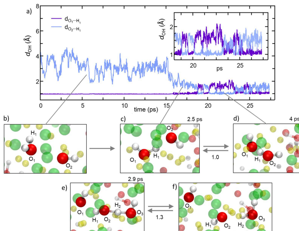
Fig. 10 (Color online) For the \text{Na}_2\text{OHCl} system: proton hopping process by which H atoms migrate through a dynamical switch between \sigma - and hydrogen-bonds giving rise to the formation of metastable water molecules (i.e. Grotthuss-like mechanism). 77–82 a) Temporal evolution of the interatomic distance between one H atom labelled \text{H}_1 atom, belonging to a water molecule initially formed, and its bonded O atom labelled \text{O}_1 . Also shown is the temporal evolution of the distance between \text{H}_1 and a second O atom labelled \text{O}_2 that is part of a neighboring hydroxyl group. Inset: zoom-in on the temporal window along which \text{H}_1 is shared between two \text{O}_1 and \text{O}_2 , leading to the transient formation and breaking of OH bond and water molecules. b-f) Inter-unit transitions between structural units in amorphous \text{Na}_2\text{OHCl} at 300 K. Indicatively, the mean lifetimes of the transient H-bonds and water molecules are reported on top of the panels whereas the transition rates are reported between the panels. Here, the transition rate is defined as the number of inter-unit transitions per ps observed within a given process (H-bond or water molecules formation). Color legend: Na, yellow; O, red, and Cl green.
