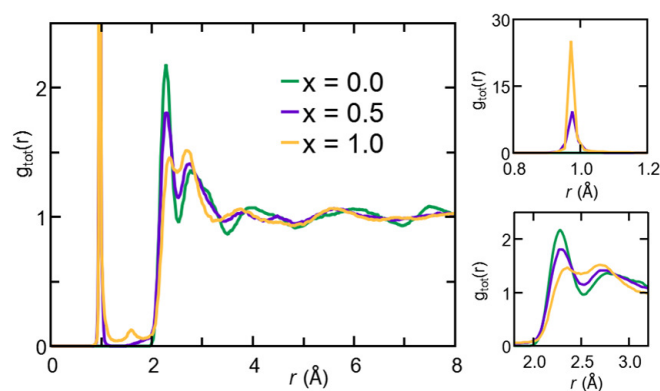
Fig. 3 (Color online) Left: Total pair correlation functions for amorphous \text{Na}_{3-x}\text{OH}_x\text{Cl} ( x=0, x=0.5, x=1 ) obtained at T=300 K. Right: Zoom-in into the 0.8\text{--}1.2 (top) and 1.8\text{--}3.2 (bottom) ranges.
