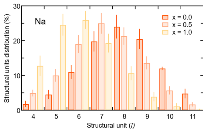
Fig. 6 Distributions of the structural units for Na of amorphous \text{Na}_{3-x}\text{OH}_x\text{Cl} ( x = 0 , x = 0.5 , x = 1 ) as a function of the number of neighbors in each unit ( l ). Values obtained by using the definition of "total" coordination n_{ij}^p , given in Sec. 3.1.3.
