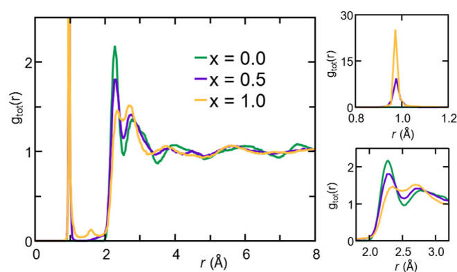
Fig. 3 (Color online) Left: Total pair correlation functions for amorphous \text{Na}_{3-x}\text{OH}_x\text{Cl} ( x=0, x=0.5, x=1 ) obtained at T=300\text{ K} . Right: Zoom-into the 0.8\text{--}1.2 (top) and 1.8\text{--}3.2 (bottom) ranges.
