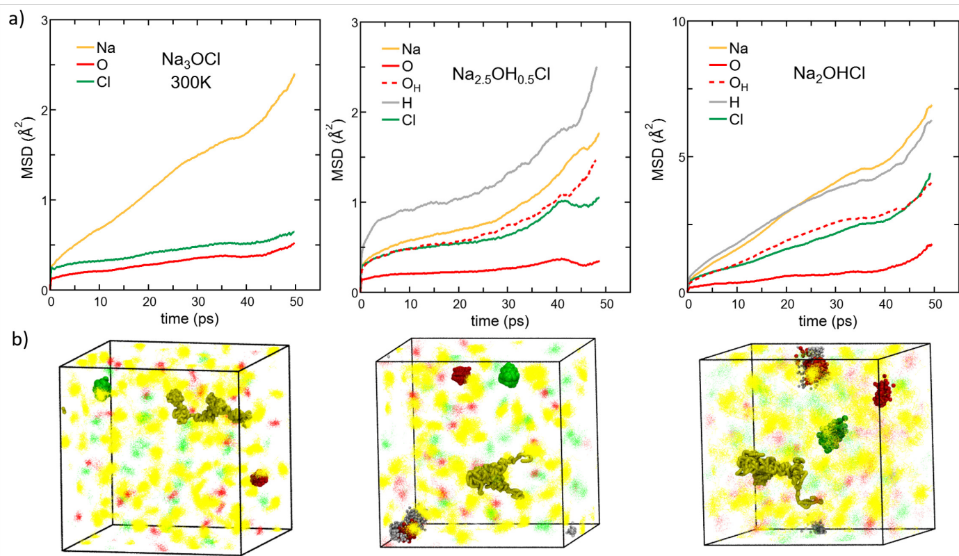
Fig. 8 (Color online) a) MSD versus time for each element in amorphous \text{Na}_{3-x}\text{OH}_x\text{Cl} ( x=0 , x=0.5 , x=1 ) at T = 300 K. Colors legend: Na, yellow; O non-bonded to H atoms, red (solid line); O bonded to H atoms, red (dashed line); H, grey; Cl, green. Note that the MSD calculated at the temperatures T=300 K, T=450 K, T=600 K, T=800 K, T=1000 K are reported in the ESI, (Fig. S1). b) Density plots \sim 50 ps trajectories of all elements are shown as dots for the three models simulated at 300 K. Na, O, and Cl atoms positions are given in yellow, red, and green, respectively. H atoms are omitted for clarity. Examples of an individual local Na migration path and Cl, O and OH local vibrations are highlighted in spheres.
