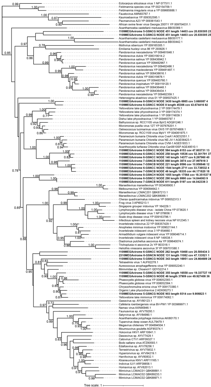
Figure S9. Putative Nucleocyotoviricota phylogeny based on the ATPase gene. Reference sequences were downloaded by NCBI GenBank (accession numbers as indicated) and sequenced recovered from the HRAP are included (in bold). Bootstrap values above 0.70 are displayed.
