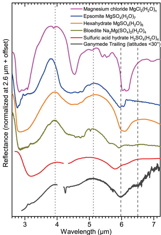
Fig. 24. Laboratory reflectance spectra of several hydrated salts and sulfuric acid hydrates. They are possibly present on Ganymede according to previous near-infrared observations ( Ligier et al. 2019 ; King & Fletcher 2022 ). The spectrum of Magnesium chloride ( <250 \mu\text{m} , JB-JLB-G32-A) is from the NASA Reflectance Experiment Laboratory (RELAB) spectral database. Spectrum of Epsomite (GDS149) is from the USGS Spectral Library ( Kokaly et al. 2017 ). Spectra of Bloedite ( \sim 250 \mu\text{m} , Jim Crowley, USGS) and Hexahydrate ( <45 \mu\text{m} , SPT143) are from the database of the Centre For Terrestrial and Planetary Exploration (C-TAPE) of University Winnipeg. The spectrum of sulfuric acid tetrahydrate at 160 K is from Loeffler et al. (2011) . We note that this is a transmittance spectrum. A reflectance spectrum of Ganymede's trailing side equatorial region ( <30^\circ latitude N/S, see Fig. 26) is scaled for comparison (black line). The vertical dotted lines indicate \text{H}_2\text{O} inter-band positions in NIRSpec spectrum, and the vertical dashed lines indicate the band positions in MIRI spectrum.
