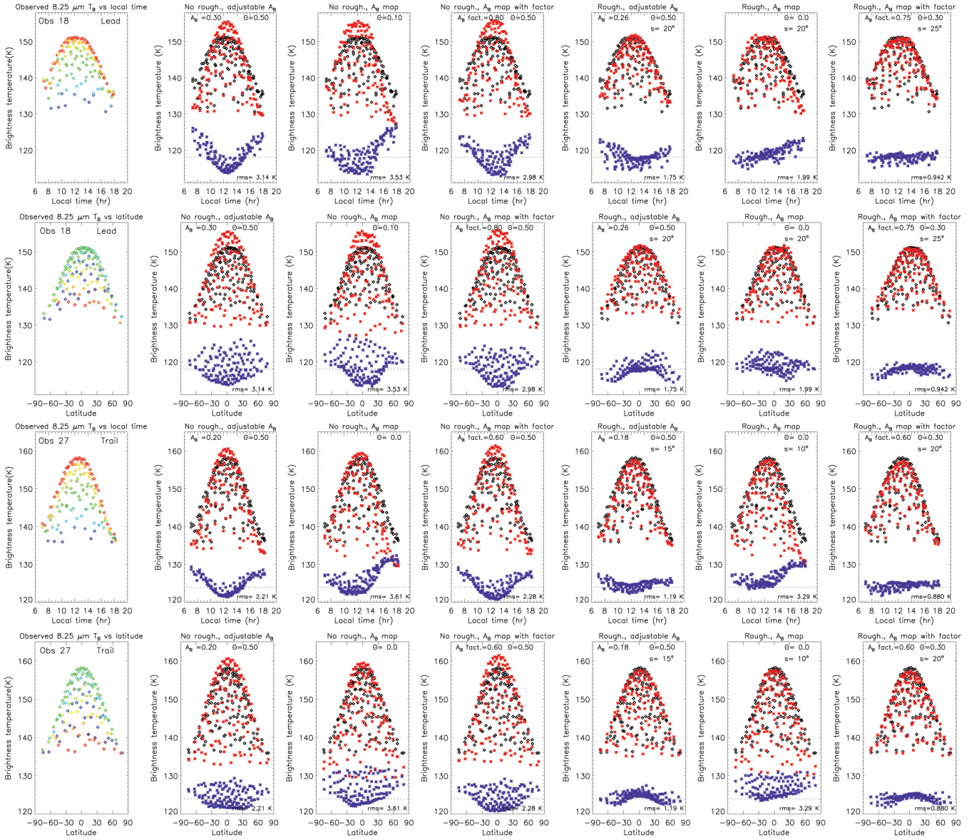
Fig. F.1. Observed and modeled 8.25- \mu\text{m} brightness temperature ( T_B ). 8.25 \mu\text{m } T_B for Obs. 18 (first two rows) and Obs. 27 (last two rows), plotted as a function of local time (first and third rows) or latitude (second and fourth rows). In each row, observational data (first column) are compared to a series of models. In the first column, the data are color-coded according to latitude (i.e., to equal values of the latitude difference from the sub-observer point) in the T_B vs local time plots, and according to local time in the T_B vs latitude plots. The following six columns describe the six considered models, with the three options for the Bond albedos and inclusion or not of surface slopes (see text for details). In those panels, data are in black, models in red, and the data minus model difference in blue, with the 0 value indicated by the dashed line. Parameter values and rms of fit are indicated in each panel.
