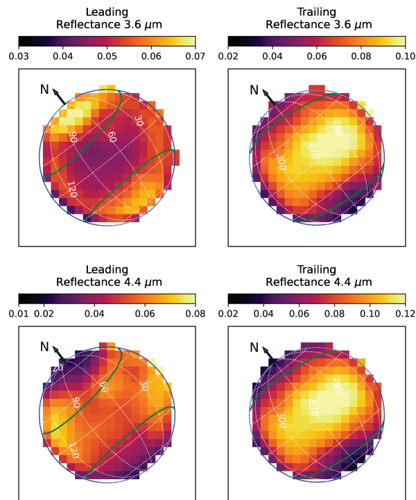
Fig. 3. Ganymede 3.6- \mu\text{m} and 4.4- \mu\text{m} reflectance maps. From top to bottom: reflectance images at 3.6 (NRS1) and 4.4 \mu\text{m} (NRS2) for Leading (left) and Trailing (right) hemispheres. Iso-latitude and longitude lines are drawn by increments of 30^\circ . The color scale is different for each map. The reflectance at the spaxels near the limb is somewhat inaccurate, as no PSF correction was applied.
