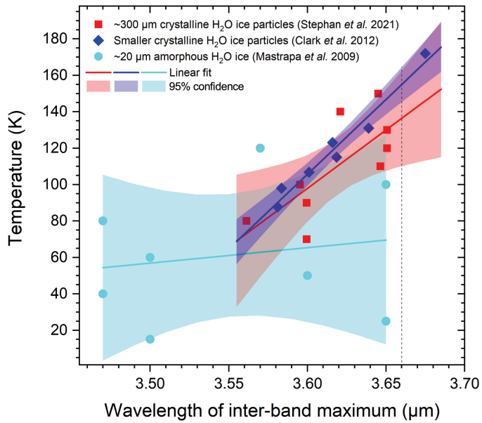
Fig. D.1. Correlation between the temperature of pure \text{H}_2\text{O} ice and the wavelength at which the reflectance bump of the 3.6\text{-}\mu\text{m} \text{H}_2\text{O} ice inter-band is maximum. For pure crystalline \text{H}_2\text{O} ice, the laboratory reflectance spectra are from Clark et al. (2012) and Stephan et al. (2021). For amorphous ice, points have been estimated by reflectance spectra with Mastrapa et al. (2009) optical constants, and applying a shift of 0.1\ \mu\text{m} .
