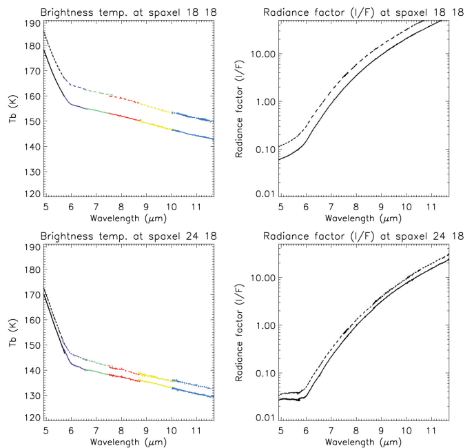
Fig. 14. Sample spectra at 4.9-11.7 \mu\text{m} from Obs. 18 (leading hemisphere, solid line) and 27 (trailing hemisphere, dashed line), at reconstructed disk center (spaxel 18, 18, top) and at offsets RA = 0.65°, DEC = 0° from this position (spaxel 24, 18, bottom). Spectra are calibrated either in brightness temperature ( T_B , left panels) with different colors illustrating different bands from 1A to 2C, or radiance factor ( I/F , right panels). They are not corrected for any account of “filling factor” associated with the fact that for positions close to limb, the PSF partly samples empty space.
