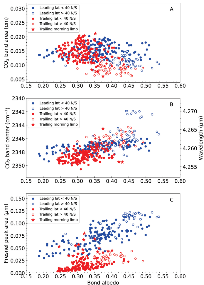
Fig. 12. CO 2 band area (A) and band center (B), and Fresnel-peak area (i.e. EqW , C) as a function of Bond albedo. Data for the Leading and Trailing hemispheres are shown with blue and red symbols, respectively. Filled and open dots are for latitudes lower and higher than 40^\circ N/S, respectively. Data in the morning limb of the Trailing hemisphere (namely longitudes > 320^\circ ) are shown with the star symbol.
