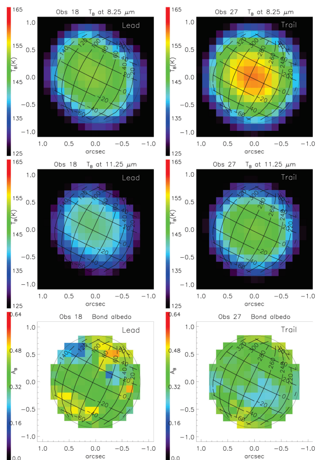
Fig. 16. Maps of the 8.25\text{-}\mu\text{m} (top) and 11.25\text{-}\mu\text{m} (middle) brightness temperature, and spaxel-averaged Bond albedo maps (bottom) from de Kleer et al. (2021) (see text). Left: leading side (Obs. 18). Right: trailing side (Obs. 27).
