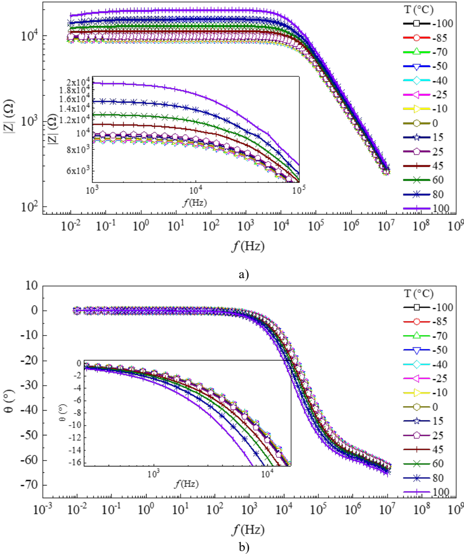
Fig. 2 Broadband impedance spectroscopy of nanocomposites at 4 wt.%. a) |Z| , b) \theta .
