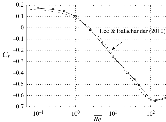
Figure 7. Predicted lift coefficient as a function of Reynolds number, \bar{Re} , for G/d = 0.005 for the uniform rolling case. The dashed line shows an empirical fit for the steady Reynolds number range provided by Lee & Balachandar (2010, equation (3.15)).
