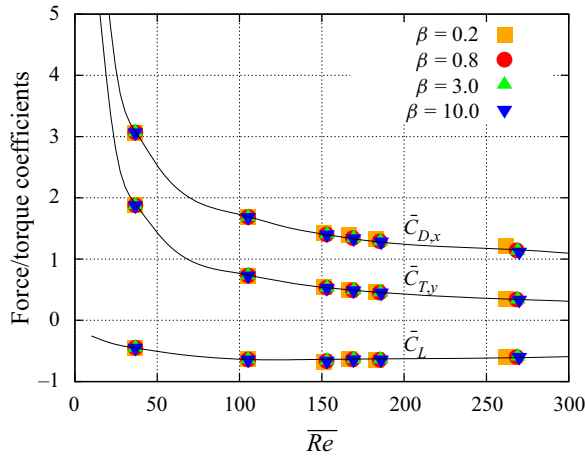
Figure 6. Predicted mean drag and lift coefficients of the freely rolling sphere, as functions of mean Reynolds number \bar{Re} for G/d = 0.005 . The solid lines represent the results for uniform rolling, i.e. rolling in a straight line at constant speed.
