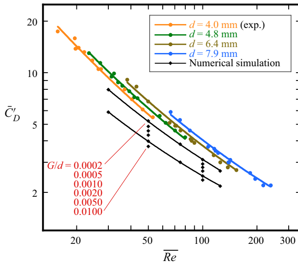
Figure 26. Close-up of the \bar{Re}-\bar{C}'_D relation for spheres of the same material (acrylic), but of different diameters, compared to the values obtained from numerical simulations using different gap ratios.
