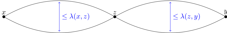
Figure 2: A cut-vertex z inside some interval I(x, y) .
