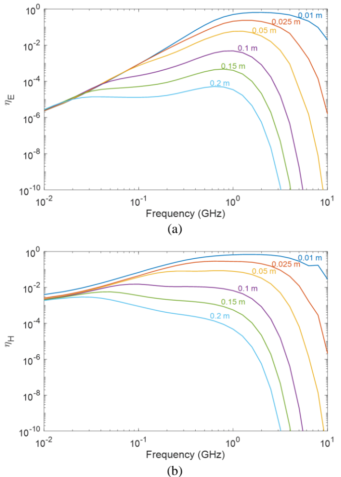
Fig. 3. Radiation efficiency for an (a) electric \eta_E and magnetic (b) \eta_H receiver as a function of the frequency and the phantom radius R_p (asymptotic to the implantation depth).
