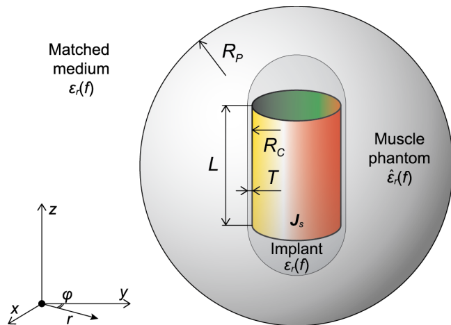
Fig. 1. Problem formulation (not to scale). The implant is centered inside of a spherical (radius R_p ) muscle-equivalent phantom {dispersive complex permittivity \epsilon_r(f) according to [14]}. The phantom is surrounded by a lossless medium with \epsilon_r(f) . The receiving electric or magnetic antenna is modelled by corresponding current distributions J_s on a cylindrical aperture. The aperture is insulated by a lossless volume with \epsilon_r(f) .
