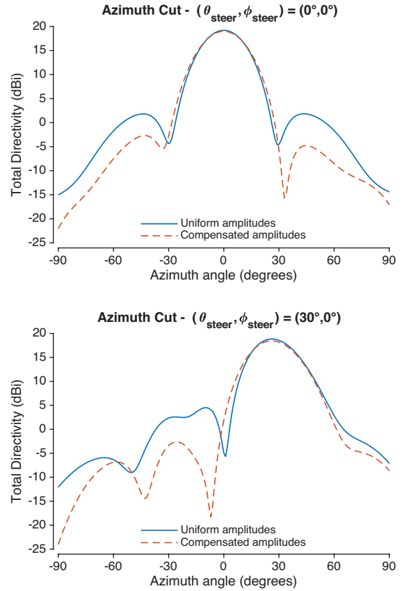
Fig. 5. Azimuthal scan of the on-body conformal array shown in Fig. 4 for 0^\circ elevation angle. The continuous blue line is the result before element switching, with all elements with unitary amplitudes, whereas the orange dashed line is the result after amplitude compensation.
