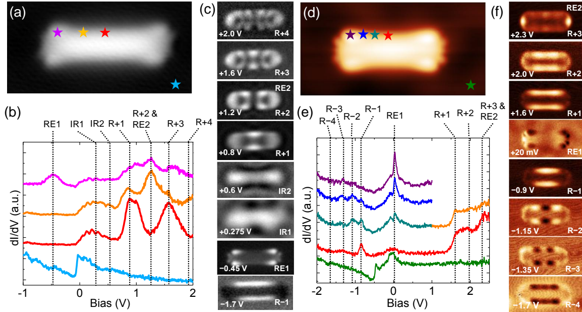
FIG. 2. Electronic tunneling excitation resonances of a 5-monomer-unit long 7-aGNR on Ag(111) and Au(111). (a) STM image of a 5-monomer-unit long 7-aGNR on Ag(111) surface ( V_{\text{bias}} = +20 mV, I = 20 pA). (b) Corresponding dI/dV spectra recorded at different positions (marked with colored stars in (a)) along the armchair side. Several electronic resonances of the 7-aGNR are resolved and highlighted with vertical dotted lines. (c) Corresponding dI/dV maps recorded at the tunneling resonance voltages revealed in (b). They showcase the electronic behavior of 7-aGNR on the Ag(111) surface. RE1 and RE2 represent the low-bias and high-bias ESs of the 7-aGNR, respectively. IR1 and IR2 represent the interface resonances. (d-f) STM image and dI/dV characteristics revealing the electronic behavior of the same length (5-monomer-unit long) 7-aGNR on the Au(111) surface similar to that on the Ag(111) surface presented in (a-c), respectively. Scan sizes are 8 \text{ nm} \times 4 \text{ nm} (length \times height). Ag(111) and Au(111) reference dI/dV spectra are presented in blue and green curves in (b) and (e), respectively.
