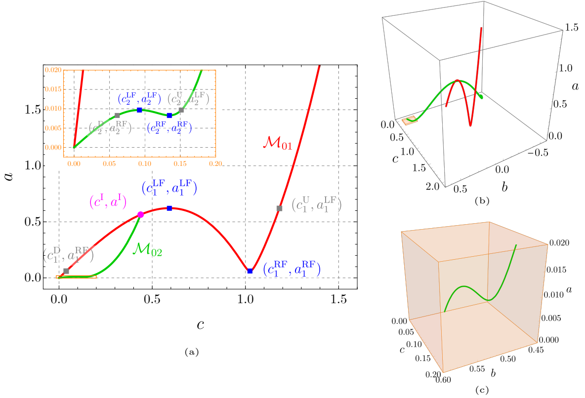
Figure 6: Typical example of the critical manifold. (a) In the (c, a) -plane. The branches a = H_1(c) ( \mathcal{M}_{01} ) and a = H_2(c) ( \mathcal{M}_{02} ) are plotted in red and green, respectively. The fold points (c_i^{\text{LF}}, a_i^{\text{LF}}) and (c_i^{\text{RF}}, a_i^{\text{RF}}) ( i = 1, 2 ) (blue points), the points (c_i^{\text{U}}, a_i^{\text{LF}}) and (c_i^{\text{D}}, a_i^{\text{RF}}) (gray points) and the point (c^{\text{I}}, a^{\text{I}}) (with a^{\text{I}} = H_1(c^{\text{I}}) = H_2(c^{\text{I}}) , see Eq. (39)) (magenta point) are also represented. A zoom is made to better see the shape of \mathcal{M}_{02} . (b) In the (b, c, a) -space. (c) Zoom of (b) corresponding to the orange colored rectangular cuboid area. The following parameters are used: \mu = 0.1 , \beta = 0.65 and \alpha = 2 .
