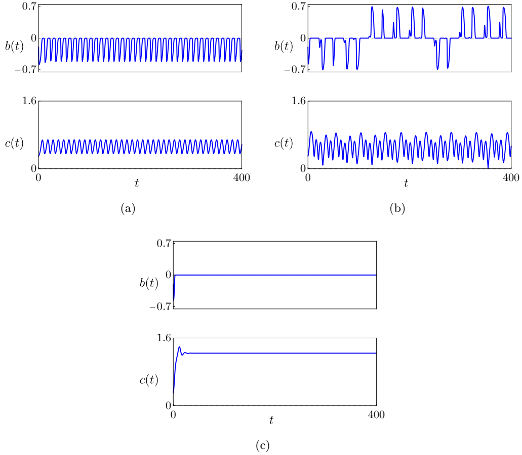
Figure 14: Numerical solutions of the fast subsystem (31) for (a) a = 0.22 , (b) 0.35 and (c) 0.45 . Parameters are the same as in Fig. 10(g) and the following initial conditions are used: b(0) = -0.2 , c(0) = 0.3 and \delta(0) = \pi .
