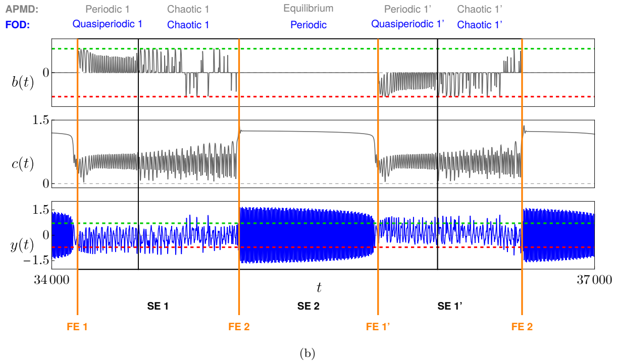
Figure 11: Same numerical simulations as in (a) Figs. 10(f) and (b) 10(g). For both (a) and (b) from top to bottom one has the time series b(t) (gray), c(t) (gray) and y(t) (blue). The equilibrium positions y_1^{\text{st}} (dashed green line) and y_2^{\text{st}} (dashed red line) are depicted in the plot of b(t) . One has APMD for amplitude-phase modulation dynamics, FOD for full order dynamics, FE for fast epoch and SE for slow epoch.
