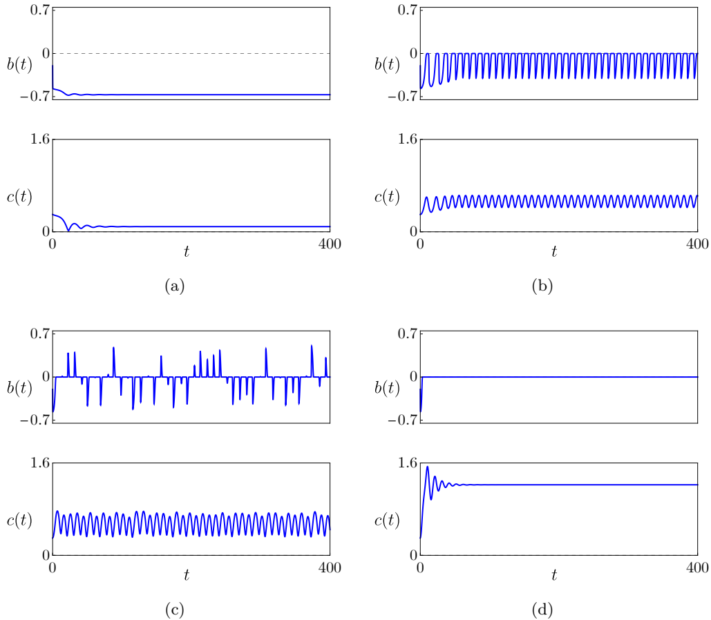
Figure 13: Numerical solutions of the fast subsystem (31) for (a) a = 0.07 , (b) 0.14 , (c) 0.25 and (d) 0.4 . Parameters are the same as in Fig. 10(f) and the following initial conditions are used: b(0) = -0.2 , c(0) = 0.3 and \delta(0) = \pi .
