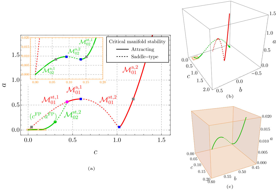
Figure 8: The different parts of the critical manifold \mathcal{M}_0 . (a) In the (c, a) -plane. For the branch \mathcal{M}_{01} (in red) one has (see Eq. (52)) from left to right: the first saddle-type branch \mathcal{M}_{01}^{st,1} , the first attracting branch \mathcal{M}_{01}^{a,1} , the second saddle-type branch \mathcal{M}_{01}^{st,2} and the second attracting branch \mathcal{M}_{01}^{a,2} . These branches are respectively connected to each other by the point p^I (magenta point) and the left and right fold points p_1^{LF} and p_1^{RF} (blue points). For the branch \mathcal{M}_{02} (in green) one has (see Eq. (53)) from left to right: the first attracting branch \mathcal{M}_{02}^{a,1} , the first saddle-type branch \mathcal{M}_{02}^{st,1} , the second attracting branch \mathcal{M}_{02}^{a,2} and the second saddle-type branch \mathcal{M}_{02}^{st,2} which ends at the point p^I . These branches are respectively connected to each other by the left and right fold points p_2^{LF} and p_2^{RF} (blue points) and the point p^{FP} (green point). (b) In the (b, c, a) -space. (c) Zoom of (b) corresponding to the orange colored rectangular cuboid area.
