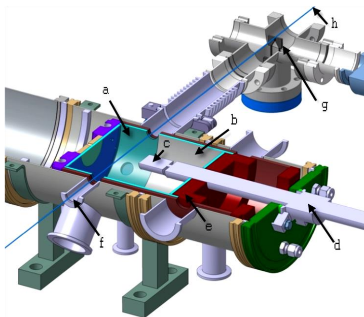
Figure 12.26. SCHEME I conceptual design (horizontal section). (a): Quartz cylinder; (b): mounted specimen; (c): permanent magnet; (d): dipolar plasma source; (e): cooling copper; (f): solar blind photoelectron multiplier tube position; (g): tuning fork – optical chopper; (h): radiation beam.
