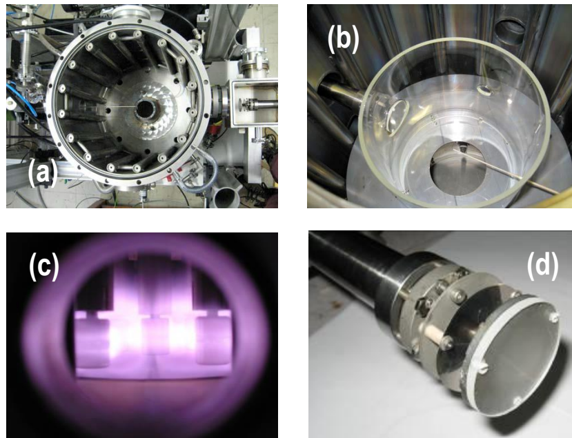
Figure 12.23. (a) The interior of the Cabembert III multi cusp chamber. (b) The Pyrex™ cylinder installed at the center of the Camembert III chamber. (c) Photo of three (out of seven) elementary plasma sources in operation. (d) Sample holder, where a Pyrex™ specimen (48 mm in diameter) is mounted.
