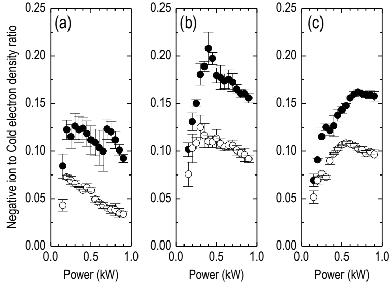
Figure 12.18. Negative ion to Cold electron density as a function of the microwave power at (a) 0.53 Pa, (b) 1.07 Pa, and (c) 1.60 Pa. Solid circles: H 2 plasma. Open circles: D 2 plasma.
