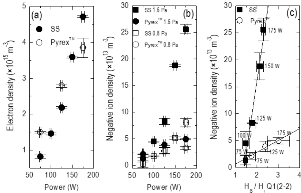
Figure 12.25. Basic plasma parameters in ROSAE III, in the cases of Pyrex™ and stainless steel (Pos. B – Fig. 12.24; single dipolar plasma source). (a) Electron density vs. power (1.6 Pa). (b) Negative ion density vs. power, at 0.8 and 1.6 Pa. (c) Negative ion density vs. the H_\beta to H_{\text{fulcher}} Q_1(2-2) intensity ratio, at different power levels (1.6 Pa).
