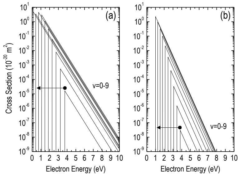
Figure 12.7. Cross section of the DEA reactions in the case of (a) H_2 and (b) D_2 . The curves are plotted according to the available data Tables in Ref. [Celiberto et al. 2001].
