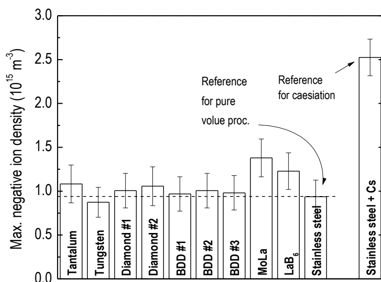
Figure 12.22. Maximal measured negative ion density for different materials at the same external experimental conditions: measured in a distance of 2.5 cm to unbiased samples, at 0.3 Pa H 2 pressure and 300 W discharge power. Redrawn from [Kurutz et al. 2017].
