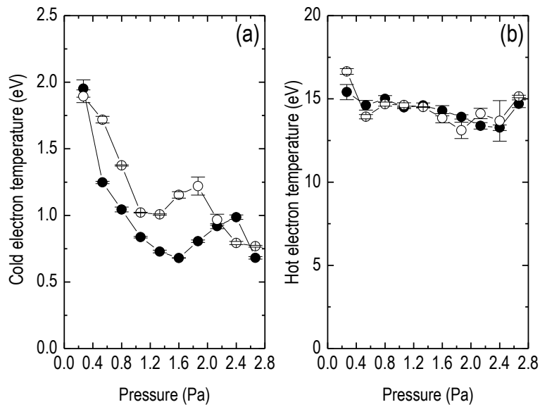
Figure 12.13. (a) Cold and (b) hot electron temperature versus the operating gas pressure [Mitrou et al. 2021]. ● H 2 ; ○ D 2 ; 0.9 kW.
