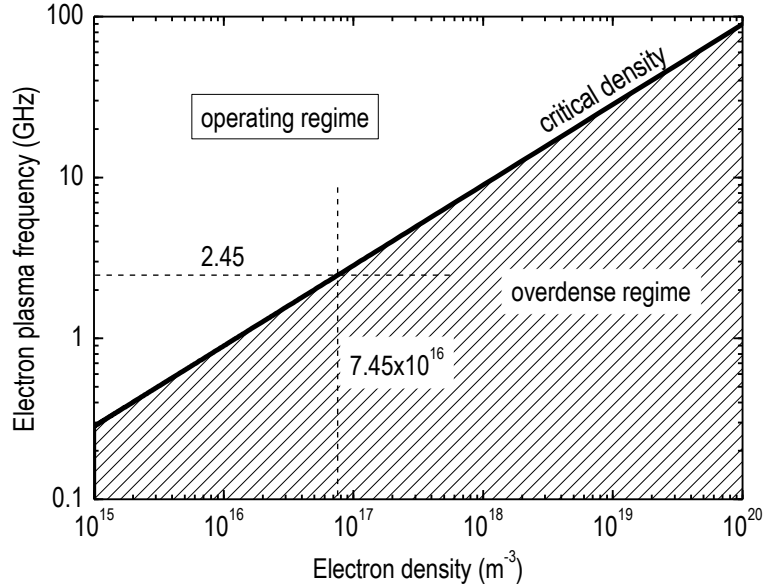
Figure 12.1. The solid line indicates the critical electron number density for different electron plasma frequencies. The widely used industrial frequency of 2.45 GHz is indicated and corresponds to a density of 7.45 \times 10^{16} \text{ m}^{-3} . Over-dense plasmas are those below and to the right of the critical density. Redrawn from [Roth 1995].
