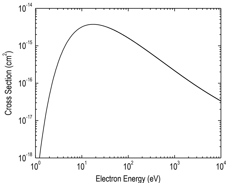
Figure 12.9. Cross section of the electron detachment (ED) reaction in hydrogen, according to analytic fit equation [Janev et al. 2003].
