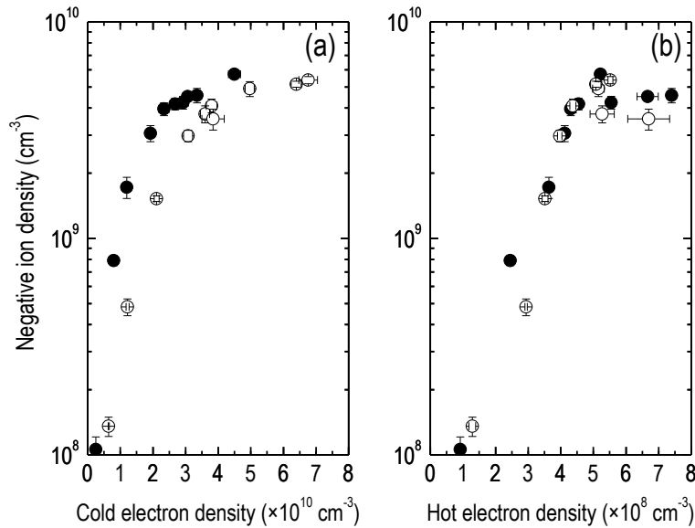
Figure 12.16. H^- and D^- ion density versus (a) cold and (b) hot electron density. Data pairs are created with the pressure elimination [Mitrou et al. 2021]. ● H_2 ; ○ D_2 ; 0.9 kW.
