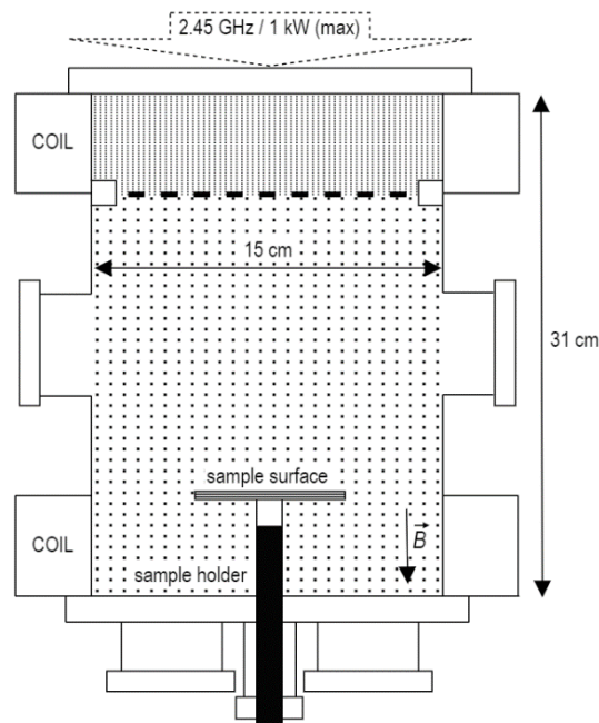
Figure 12.21. Concept of the basic version of the small scale, test bed HOMER. Redrawn from [Kurutz and Fantz 2015].
