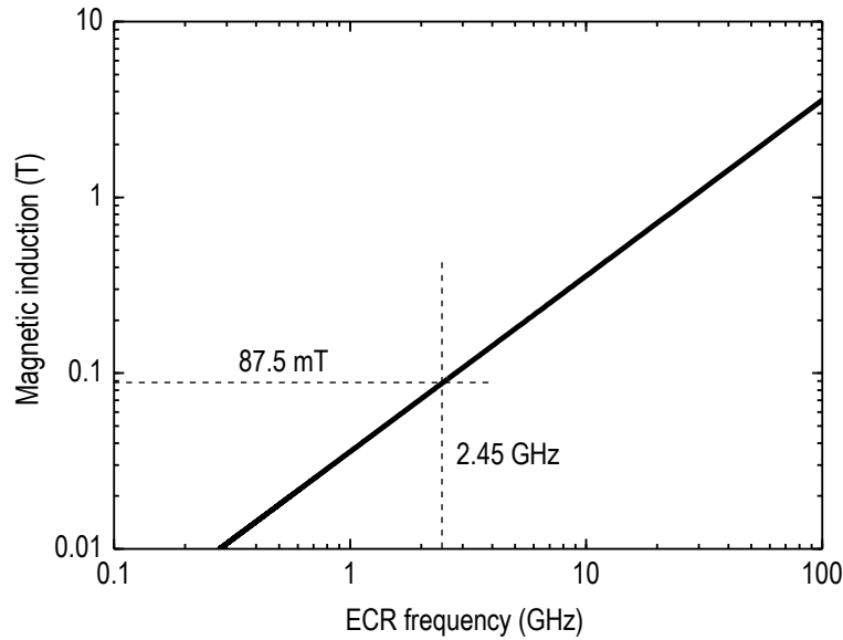
Figure 12.2. Magnetic induction requirement for fulfilling the ECR condition (Eq. 4) at different frequencies. The conventionally pair (2.45 GHz, 87.5 mT) is marked on the plot. Redrawn from [Roth 1995].
