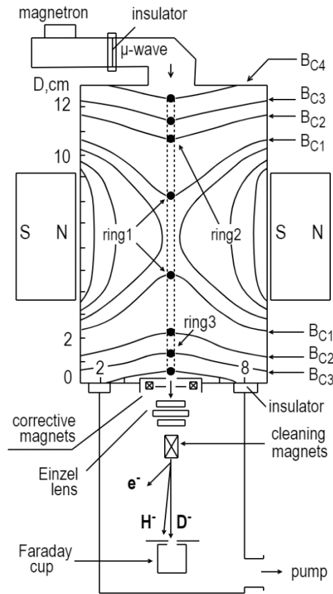
Figure 12.19. Assembly of the discharge chamber with the extraction system, concerning the ECR source with stratified plasma. Redrawn from [Dougár-Jabon 2001].
