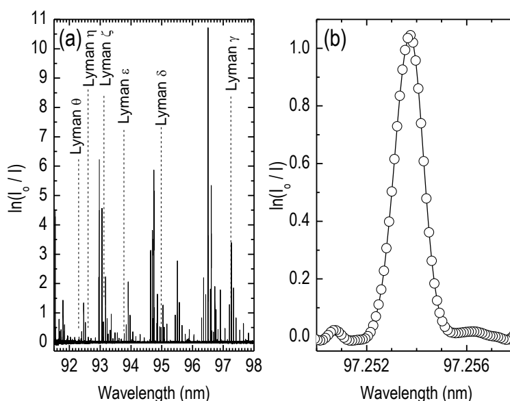
Figure 12.30. (a) Optical depth of H(n=1) obtained at 150 W and 0.8 Pa, using Quartz in the SCHEME II+ reactor. (b) Focus on the Lyman- \gamma transition.
