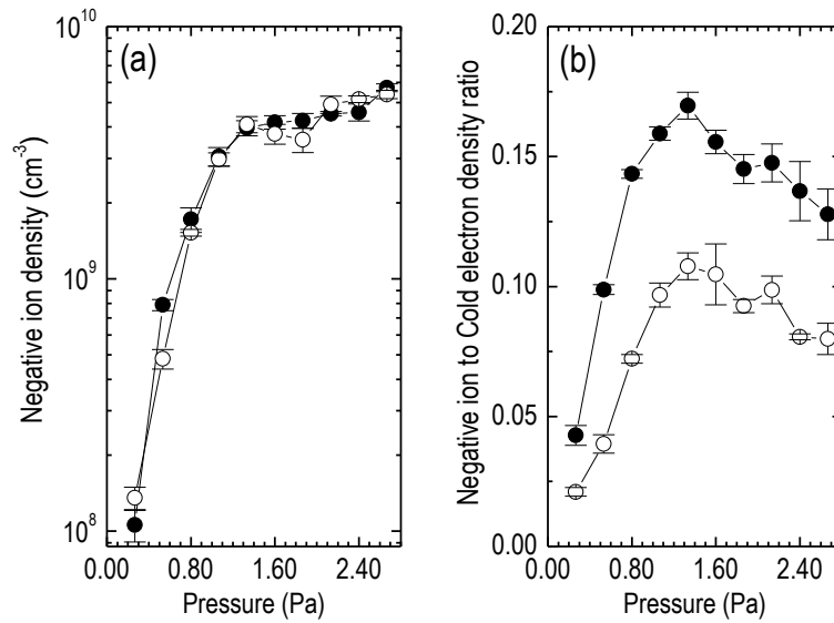
Figure 12.15: (a) H^- and D^- ion density and (b) H^- and D^- ion to cold electron density ratio, versus the operating gas pressure [Mitrou et al. 2021]. ● H_2 ; ○ D_2 ; 0.9 kW.
