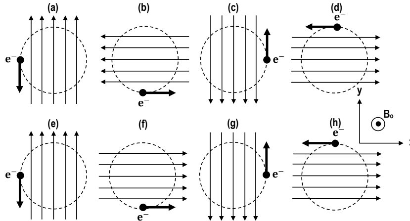
Figure 12.3. Basic principle of ECR heating. (a) – (d) Continuous energy gain for the RHP. (e) – (h) Oscillating energy for LHP: (e) gain; (f) loss; (g) gain; (h) loss. Redrawn from [Lieberman and Lichtenberg 2005].
