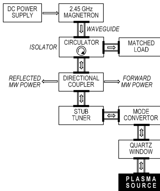
Figure 12.4. Conventional concept of the major components of an ECR-driven plasma source. The role of the individual components is discussed elsewhere [Roth 1995]. Redrawn from [Roth 1995].
