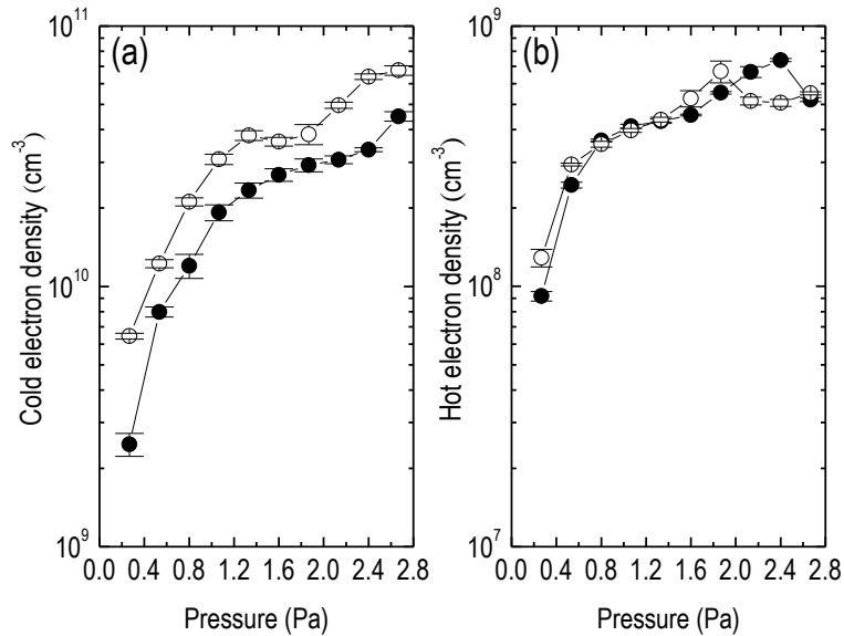
Figure 12.14. (a) Cold and (b) hot electron density versus the operating gas pressure [Mitrou et al. 2021]. ● H 2 ; ○ D 2 ; 0.9 kW.
