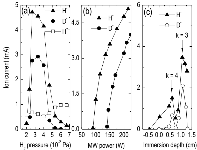
Figure 12.20 Variation of the extracted negative ion currents as a function of (a) gas pressure (200 W), (b) microwave power ( 3.33 \times 10^{-2} Pa), and (c) the immersion depth of the plasma electrode ( 2.66 \times 10^{-2} Pa; 175 W). Redrawn from [Dougarg-Jabon 2001].
