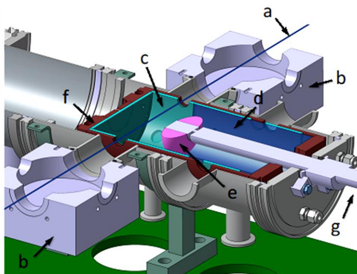
Figure 12.28. SCHEME II+ conceptual design (horizontal section). (a): radiation beam; (b): differential pumping system; (c): Quartz shell; (d): mounted specimen; (e): ECR coupling zone; (f): cooling copper; (g): dipolar plasma source.
