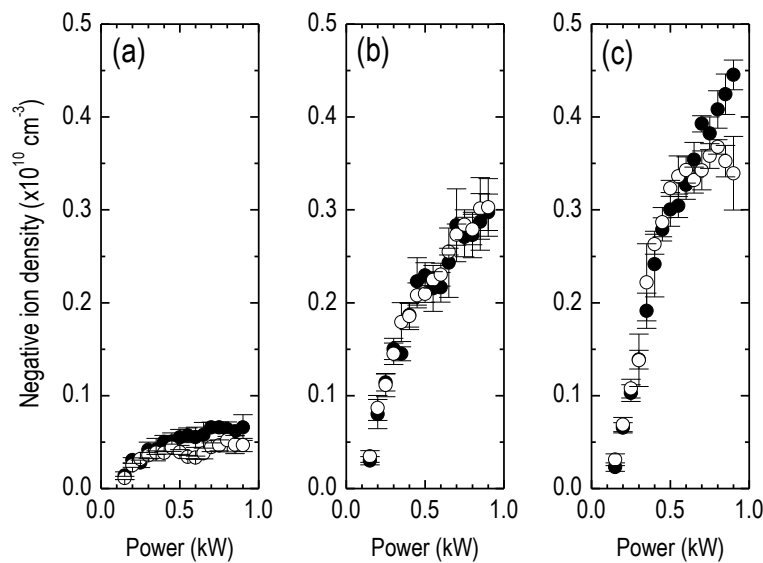
Figure 12.17. Negative ion density as a function of the microwave power at (a) 0.53 Pa, (b) 1.07 Pa, and (c) 1.60 Pa. Solid circles: H 2 plasma. Open circles: D 2 plasma.
