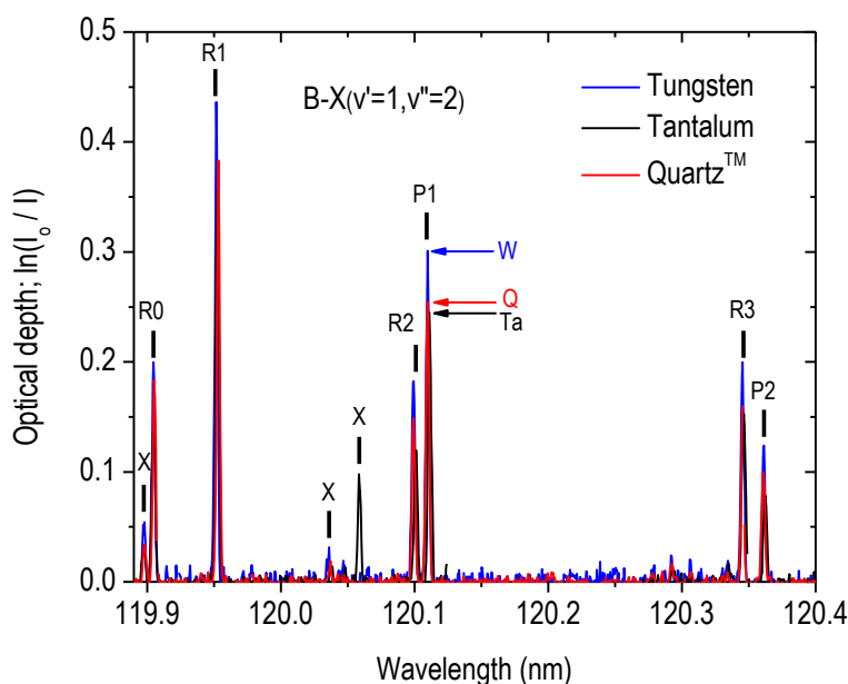
Figure 12.27. Synchrotron beam absorption spectra (optical depth) of hydrogen ECR plasma faced by three different materials: Quartz (red); Tungsten (blue); Tantalum (black). 1.6 Pa; 150 W.
