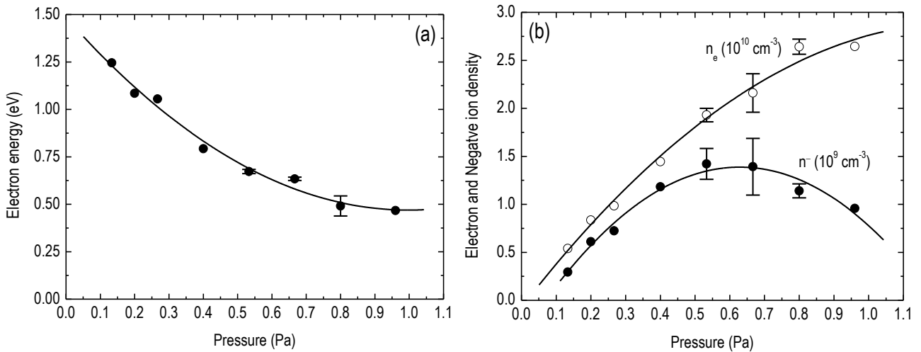
Figure 12.10. Basic plasma parameters, as a function of the operating hydrogen pressure, in the source Camembert III. (a) Cold electron energy. (b) Cold electron density ( \circ ); Negative ion \text{H}^- density ( \bullet ). Redrawn from [Svamas et al. 2006].
