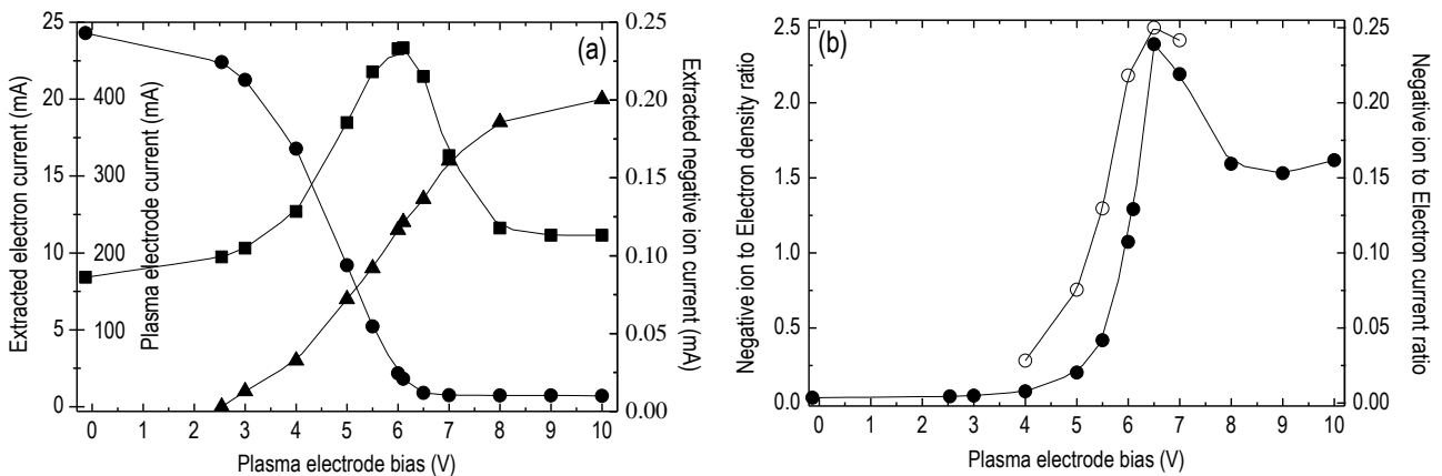
Figure 12.11. Dependence on the plasma electrode bias of the: (a) plasma electrode current ( \blacktriangle ); extracted electron current ( \bullet ); extracted negative ion current ( \blacksquare ), 0.27 Pa; (b) ratio of the negative ion to electron densities ( \circ ); ratio of the negative ion to electron extracted currents ( \bullet ), 0.27 Pa, 0.75 cm above PE. Redrawn from [Svamas et al. 2007].
