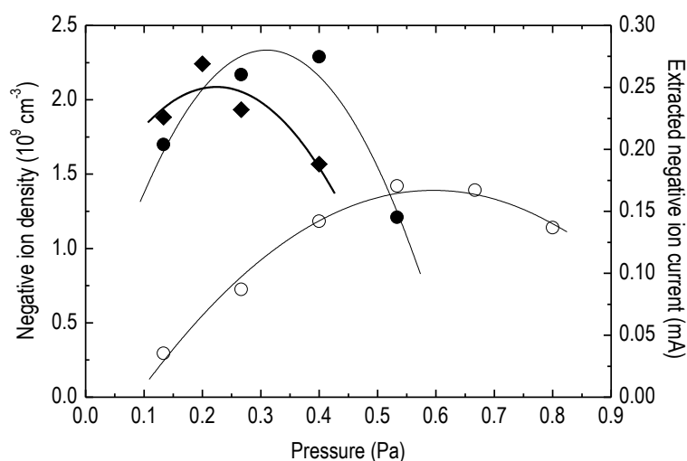
Figure 12.12. Correlation between the negative ion density and the corresponding extracted current, for variable operating pressure in hydrogen. H^- negative ion density 15 cm (○) and 0.75 cm (●) above the plasma electrode surface, and extracted negative ion current (◆). Redrawn from [Svarnas et al. 2007].
