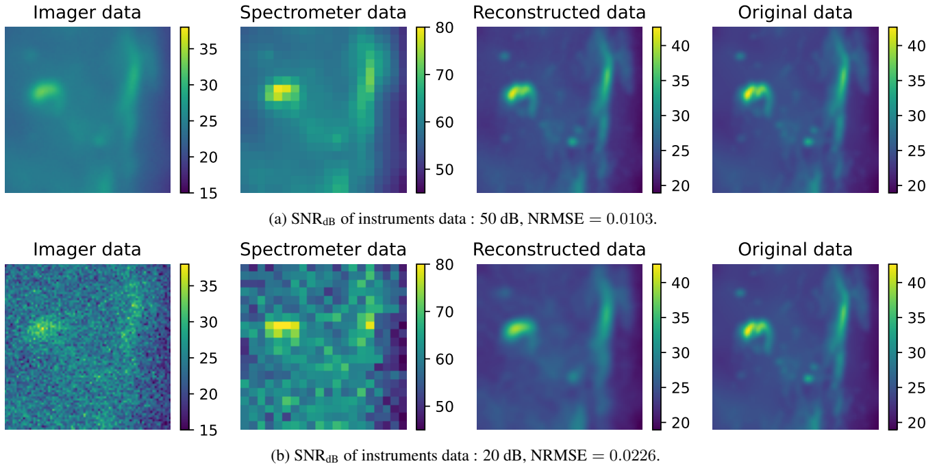
Fig. 3: Imagery data y_m at the sixth spectral band, spectrometry data y_h , reconstructed data \hat{x} , and original data x . \text{SNR}_{\text{dB}} = 50 dB for the instrument data for figure 3a, and \text{SNR}_{\text{dB}} = 20 dB for figure 3b. All images are those observed (or centered for the imager) at 15.5 \mu\text{m} . Unit in \text{mJy arcsec}^{-2} .
