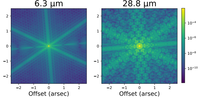
Fig. 1: MIRI PSF [7] (logarithmic scale).
