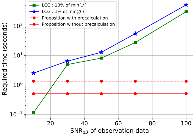
Fig. 2: Time required by the LCG algorithm to reach 10% and 1% of the minimum of the criterion \min(\mathcal{J}) (equation 11), compared with the time required by the proposed explicit solution as a function of the \text{SNR}_{\text{dB}} of the instrument data. Calculations with i9-10885H processor, 2.40 GHz (x 16), RAM 64 GB.
