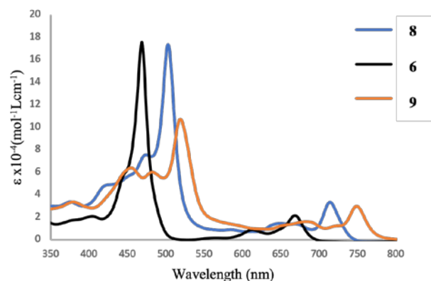
Figure 4. Electronic spectra of vanadyl(IV) porphyrin 6 and porphyrin dimers 8 and 9 (isomer \alpha - \beta ).
